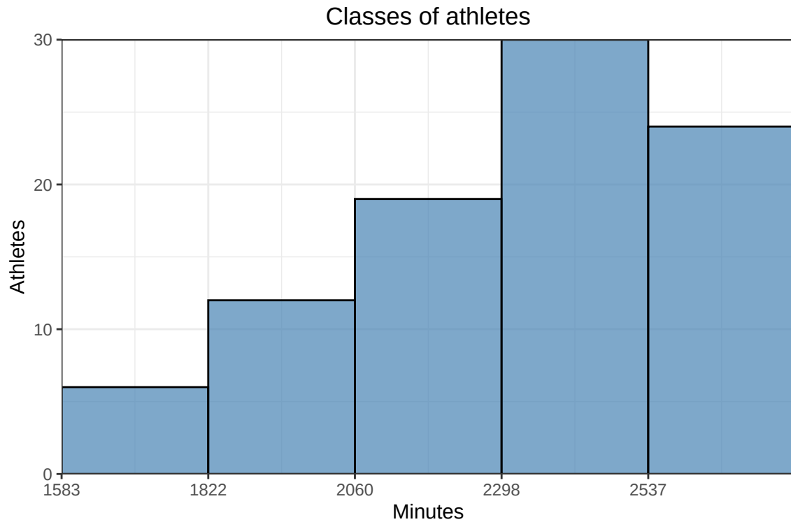
Figure 1: Distribution of finishing time in minutes for the 5 classes
