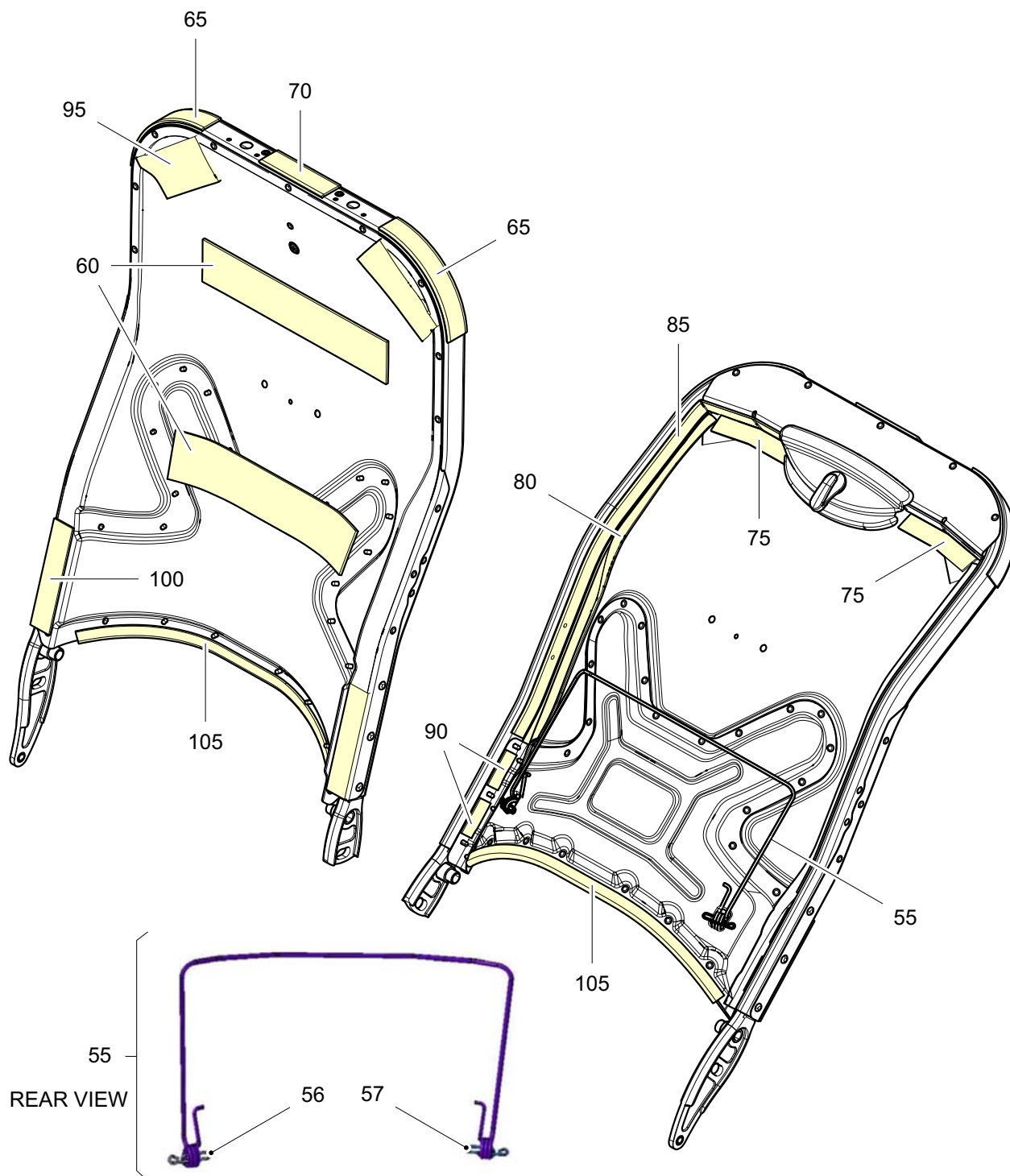
Backrest Assembly (Sheet 2 of 2)
