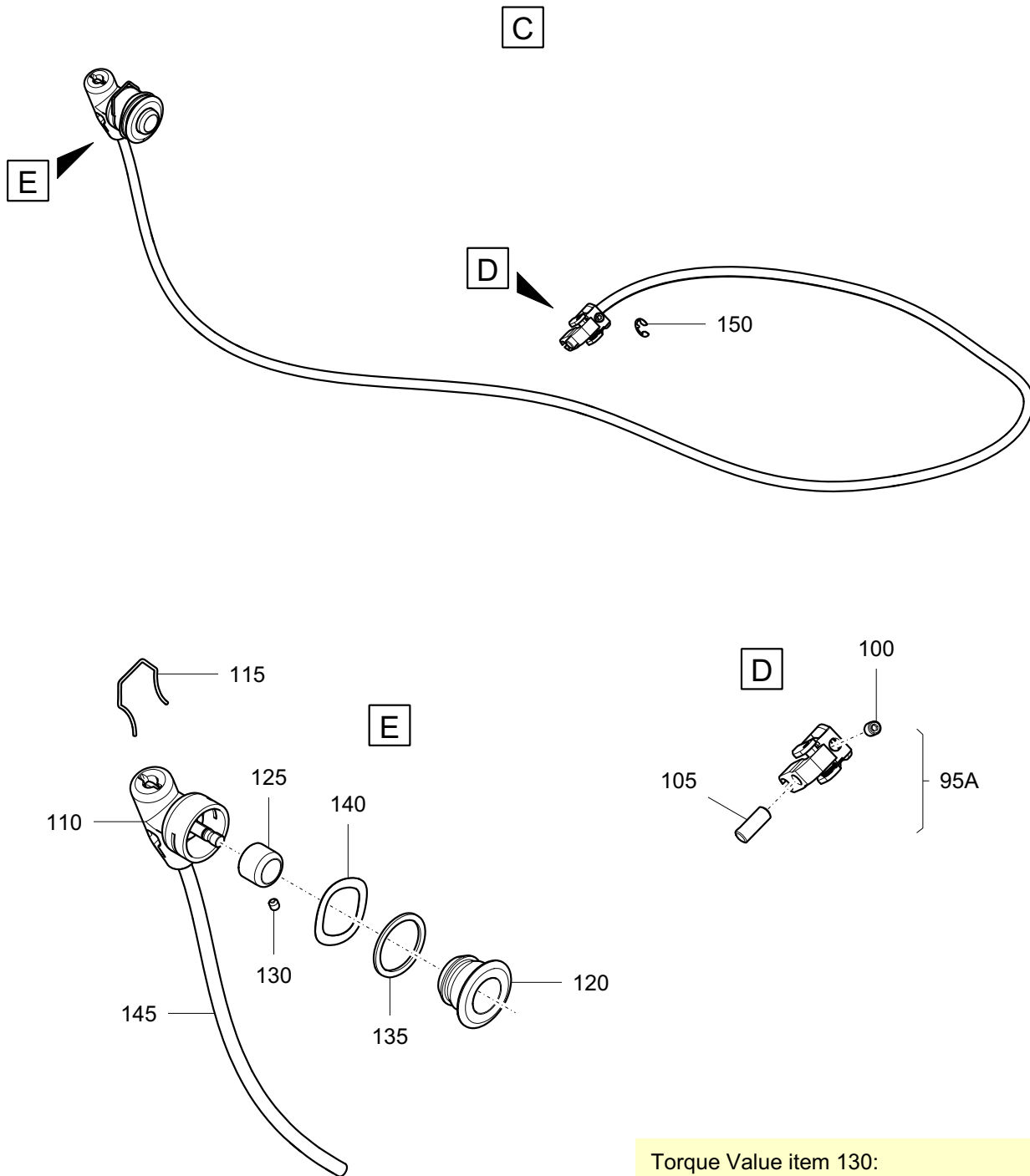
IAT Armrest Assembly (Sheet 4 of 4) Figure 5/Graphic-25-04-48-950-005-A01
