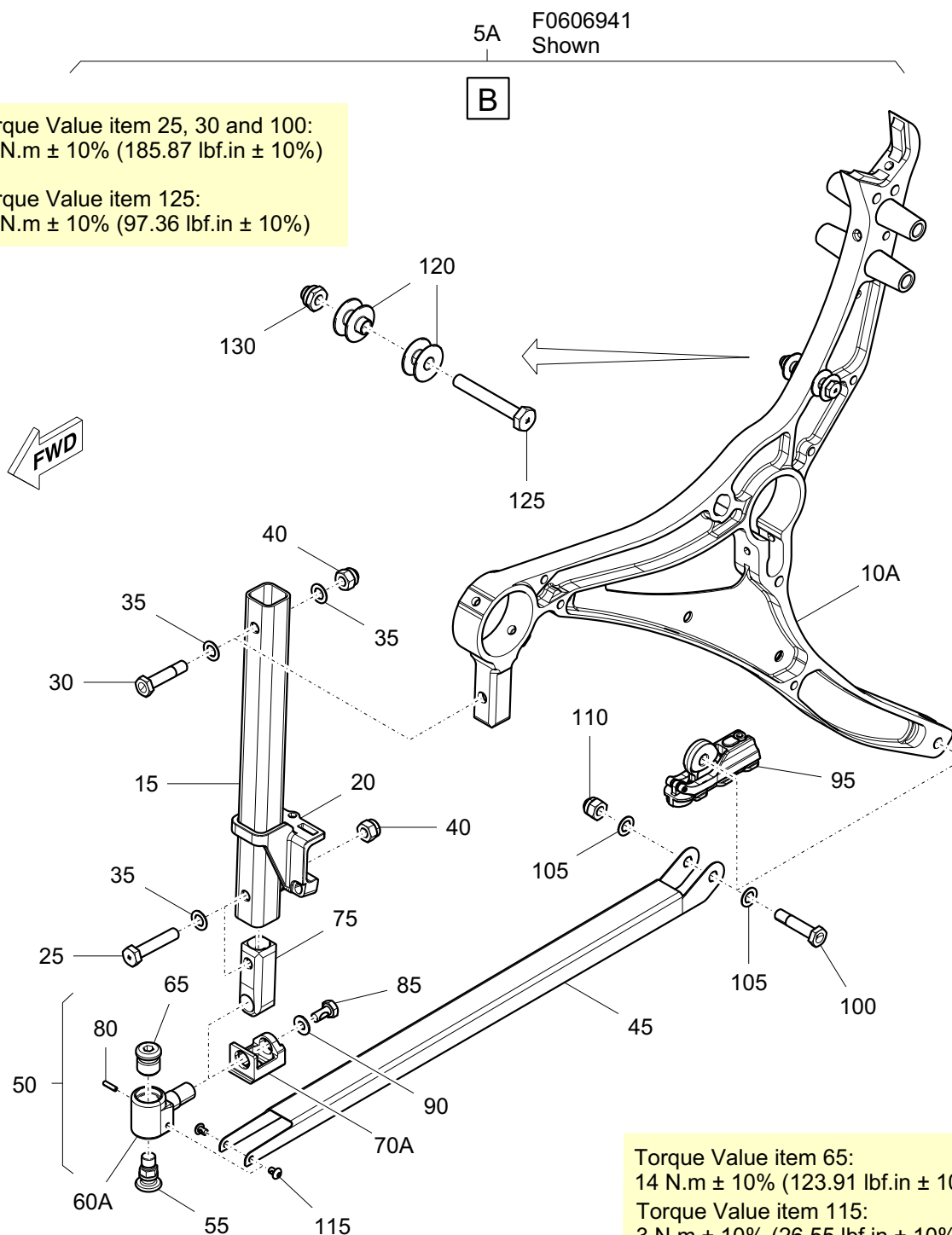
Structure Assembly (Sheet 3 of 6)
