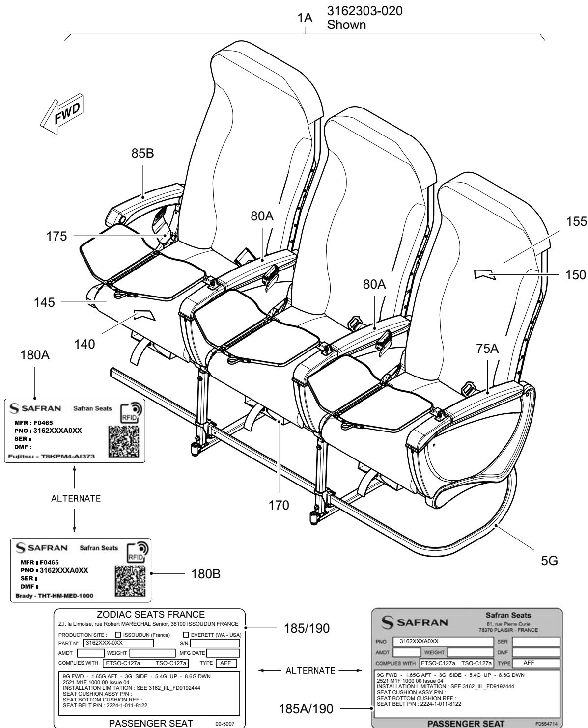
IAT Seat Assembly (Sheet 1 of 7)
