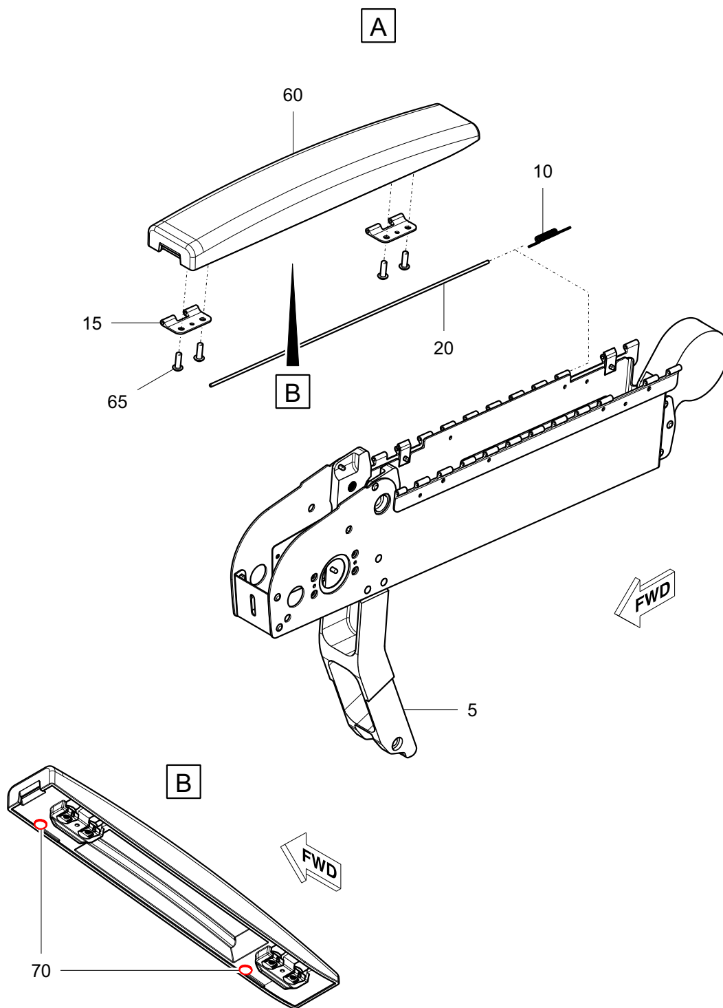
IAT Armrest Assembly (Sheet 3 of 4) Figure 5/Graphic-25-04-48-950-005-A01
