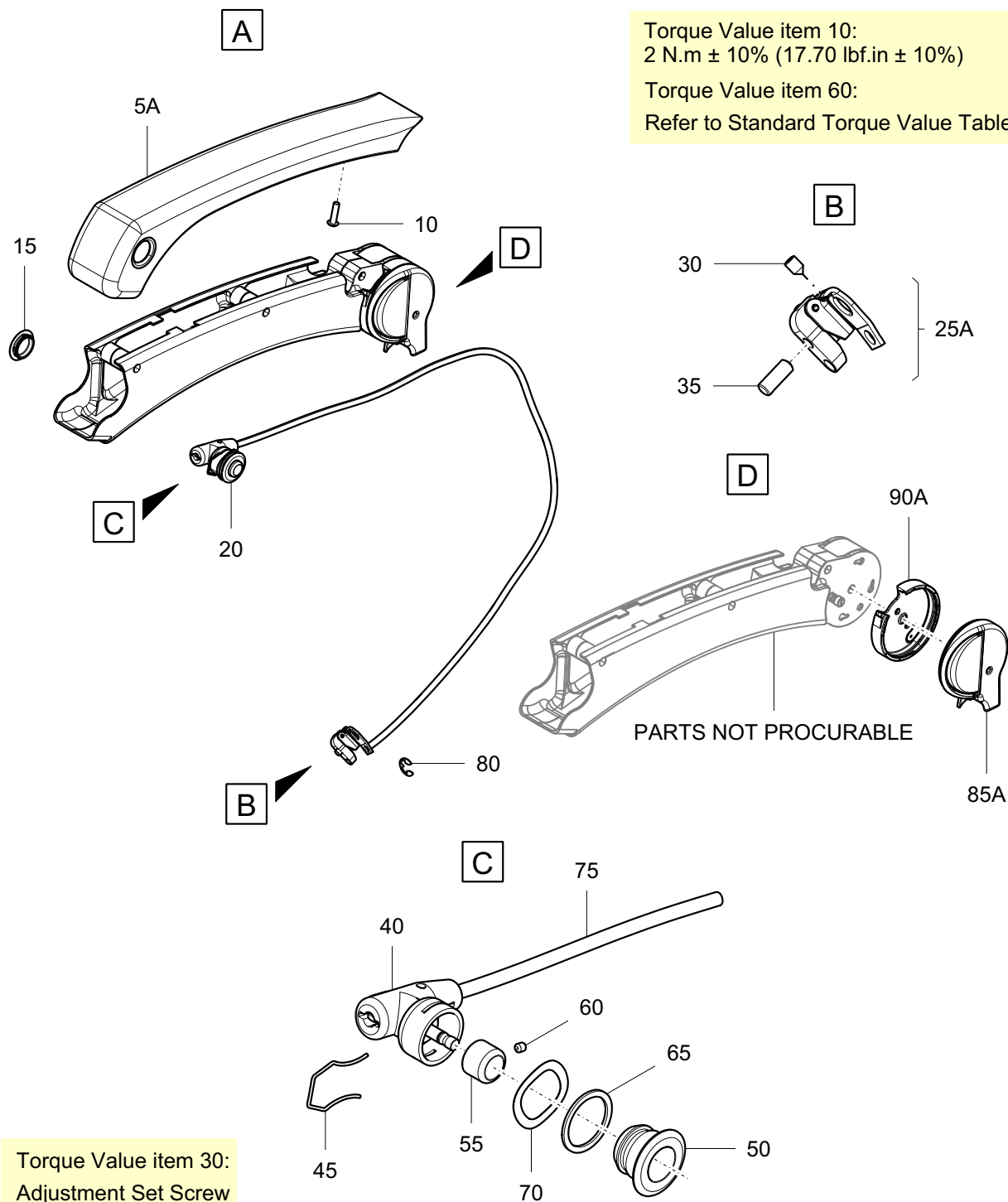
Standard Armrest Assembly (Sheet 2 of 2)
