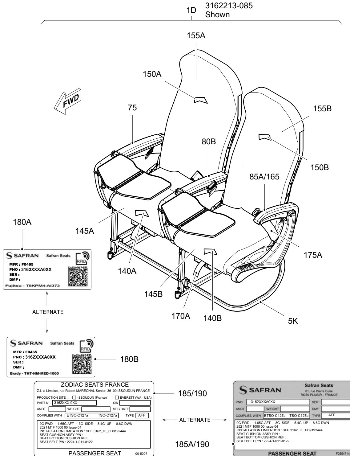
IAT Seat Assembly (Sheet 7 of 7) Figure 1A/Graphic-25-04-48-950-001-B01
