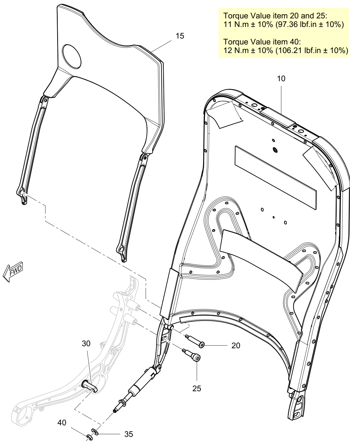
IAT Seat Assembly (Sheet 2 of 7)
