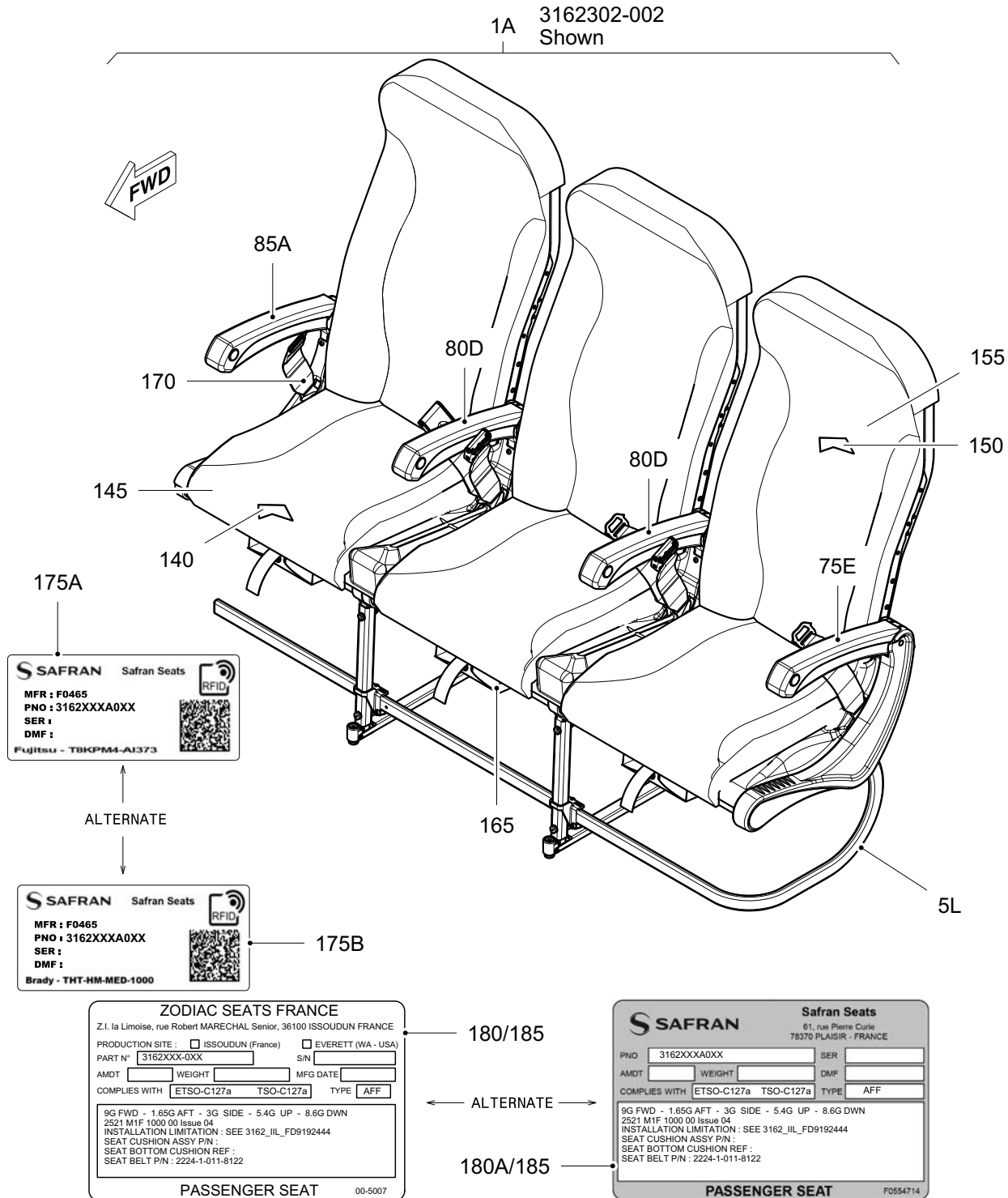
Standard Seat Assembly (Sheet 1 of 6)
