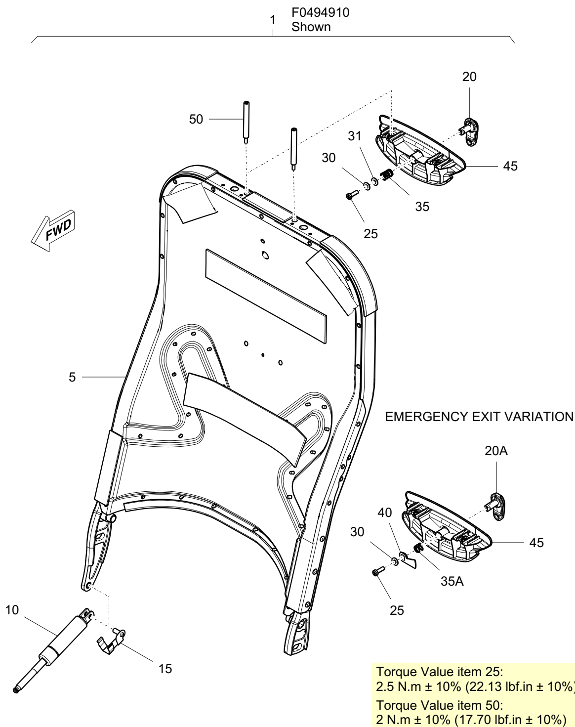
Backrest Assembly (Sheet 1 of 2)
