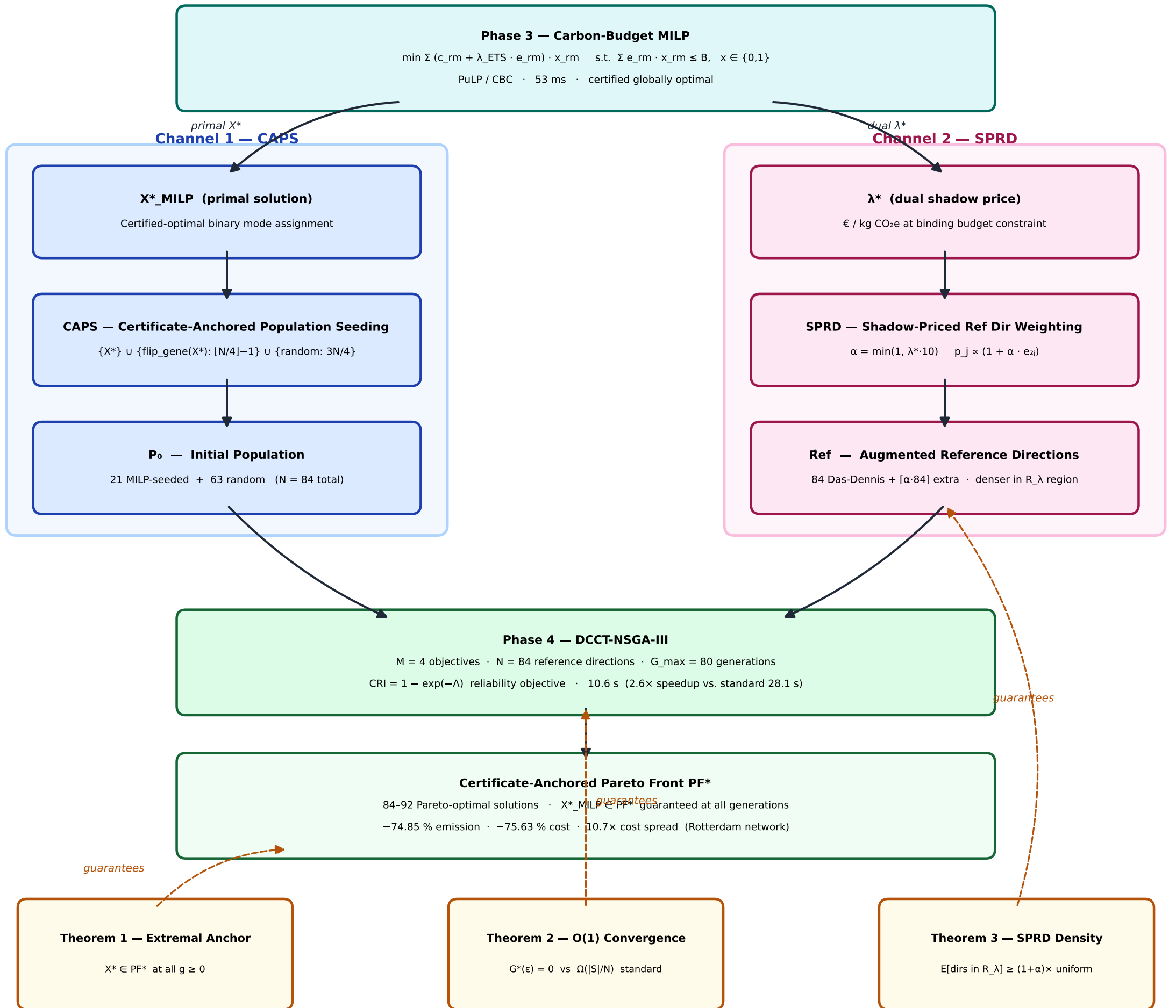
Fig. 3. DCCT dual-channel certificate transfer mechanism. Blue = Ch 1 CAPS (primal X^* ). Pink = Ch 2 SPRD (dual \lambda^* ). Dashed amber arrows = formal theorem guarantees.
