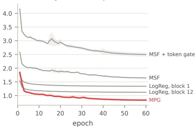
(b) Training loss (Tversky + Focal)
