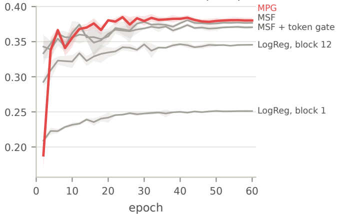
(a) Validation mean FG IoU (prompter mask)
