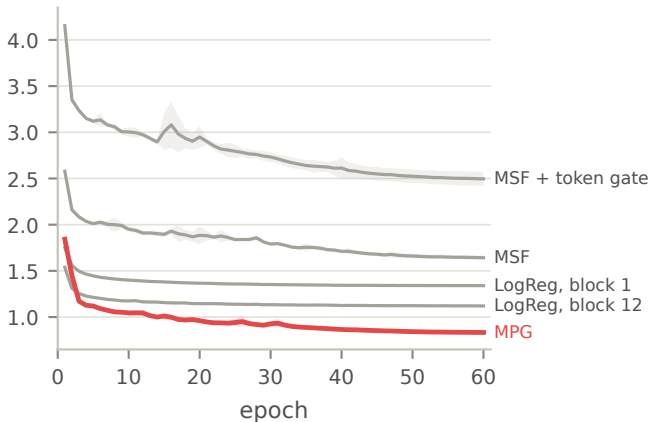
Training loss (Tversky + Focal)
