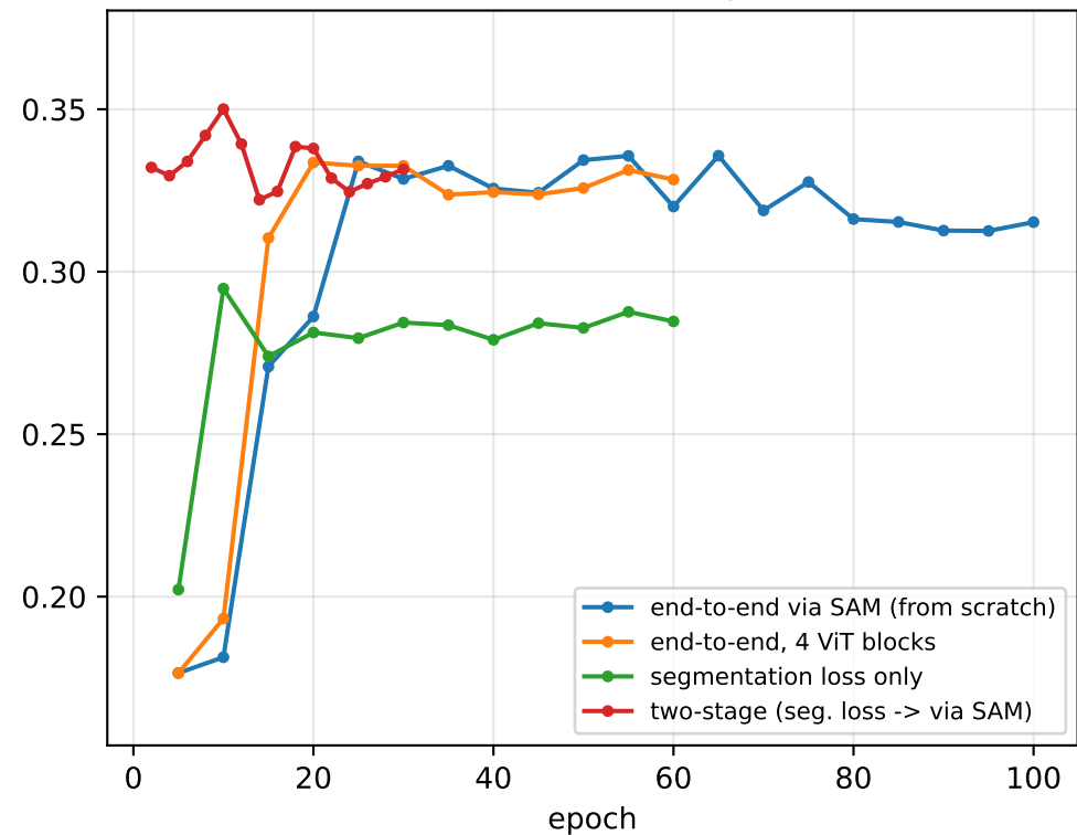
Mean FG IoU of the SAM output (test set)
