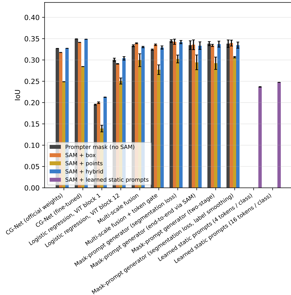
Prompter mask vs. SAM prompted by it (Infused Token, MLP ratio 1.0)
