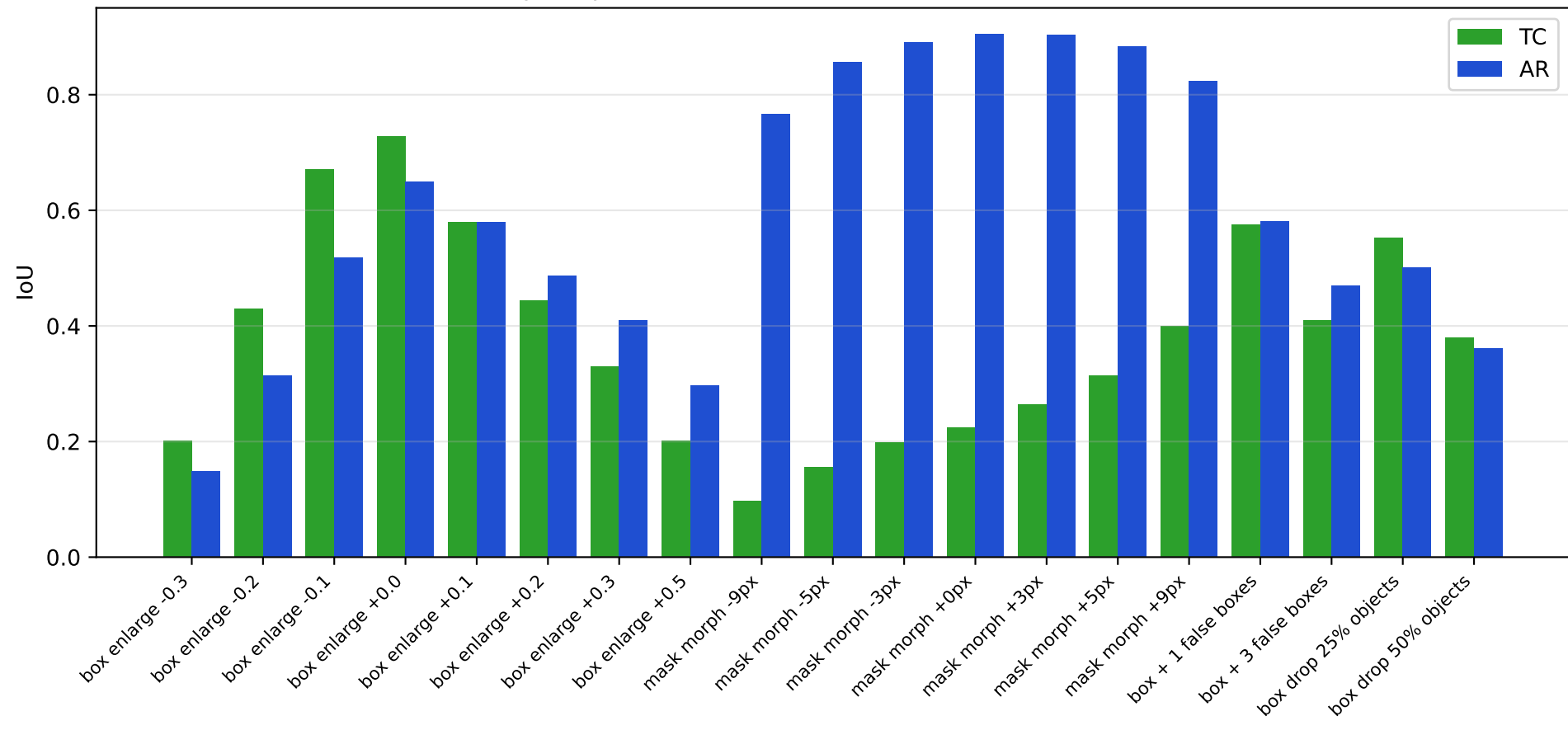
Ground-truth prompts with controlled errors (Infused Token, MLP ratio 0.5)
