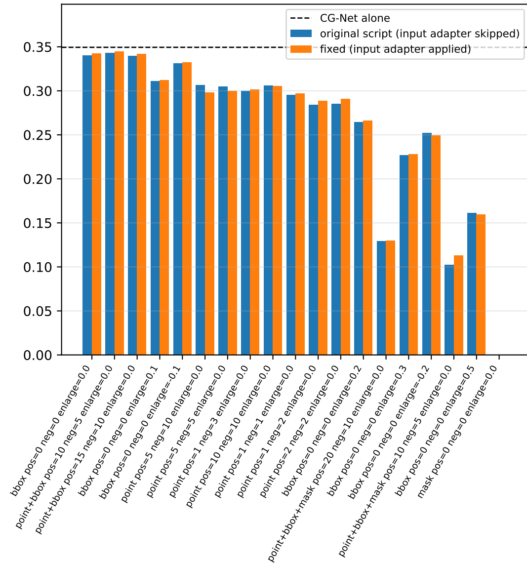
TC IoU
