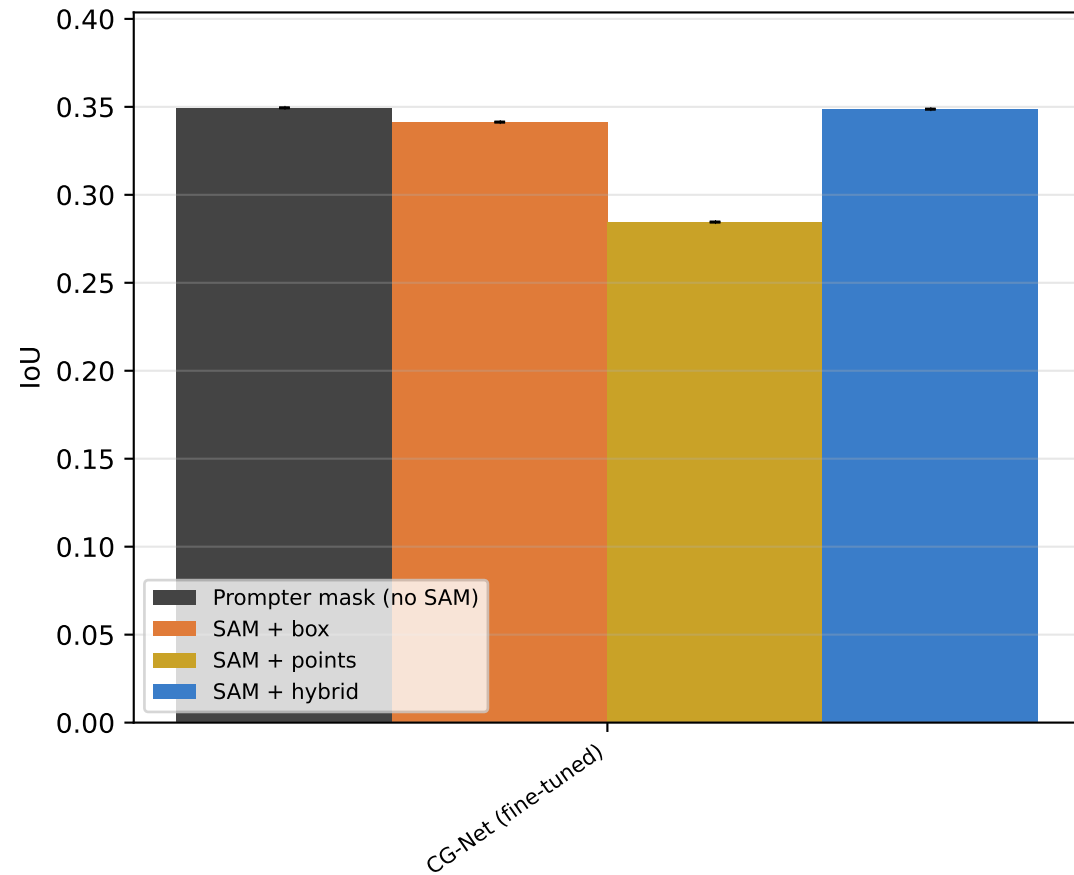
Prompter mask vs. SAM prompted by it (Infused Token, MLP ratio 1.0)
