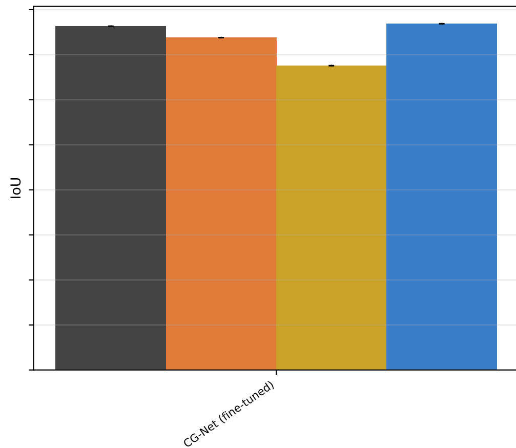
Prompter mask vs. SAM prompted by it (Infused Token, MLP ratio 1.0)
