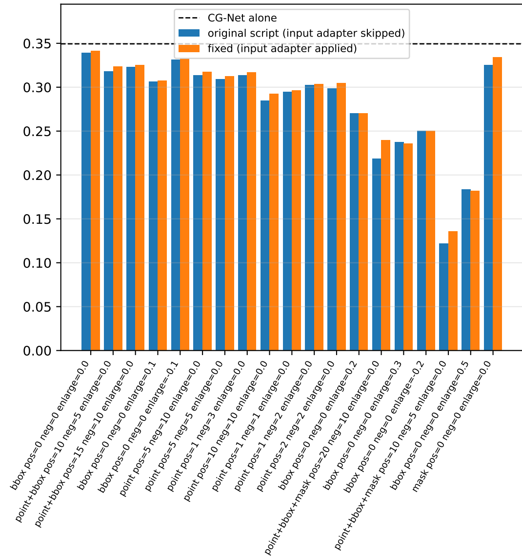
TC IoU
