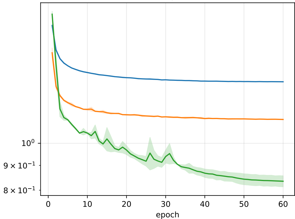
Training loss
