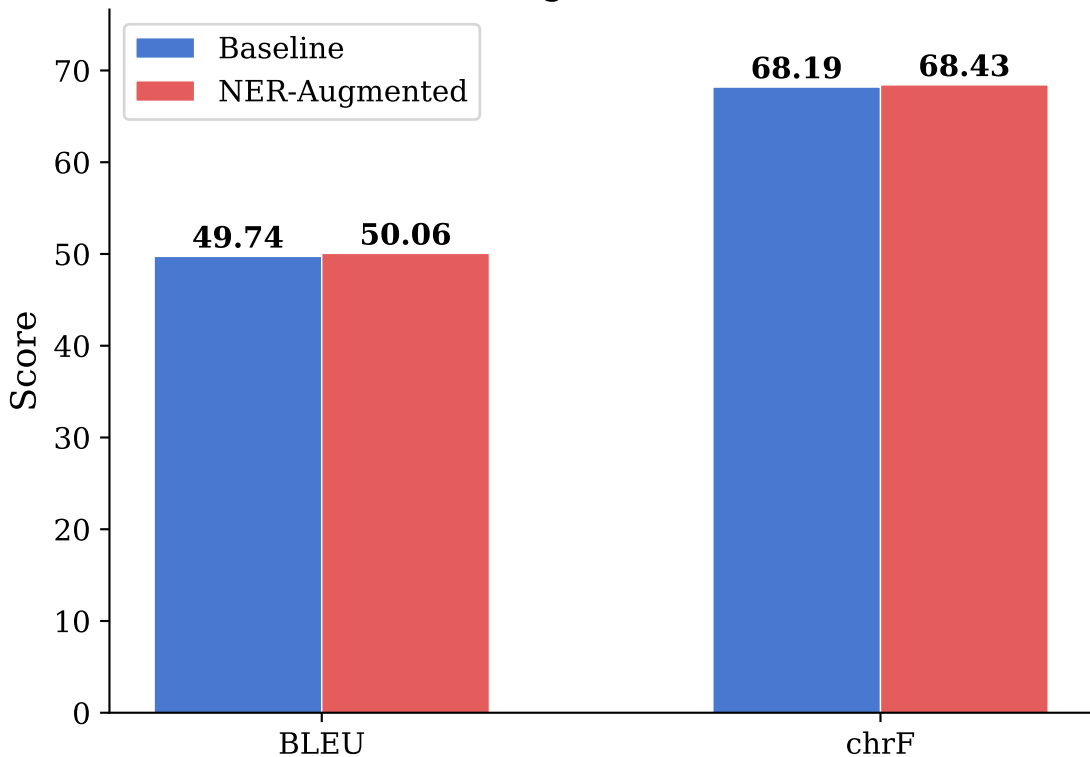
Baseline vs NER-Augmented MT Performance
