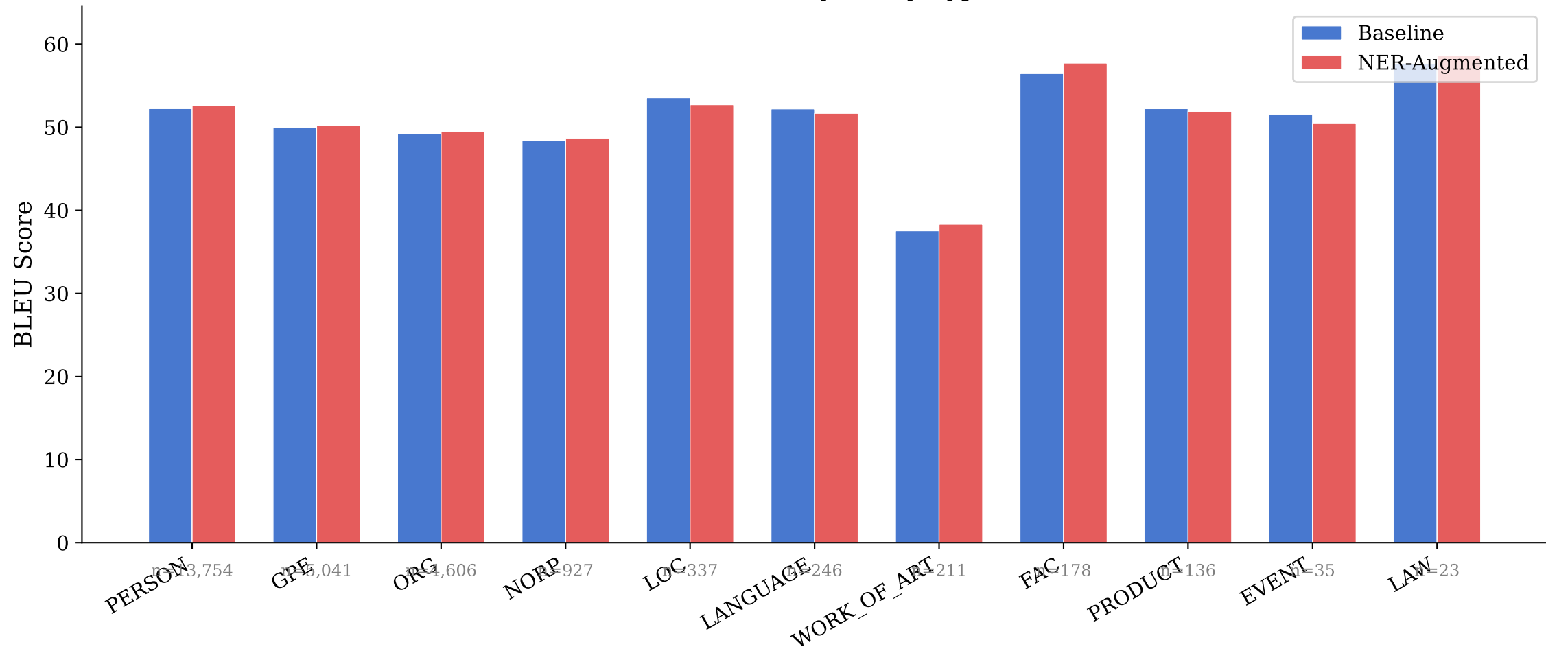
BLEU Score by Entity Type
