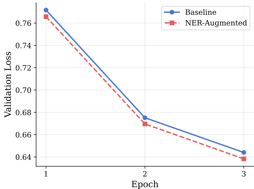
Validation Loss
