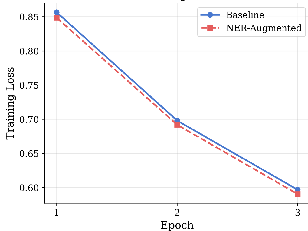
Training Loss
