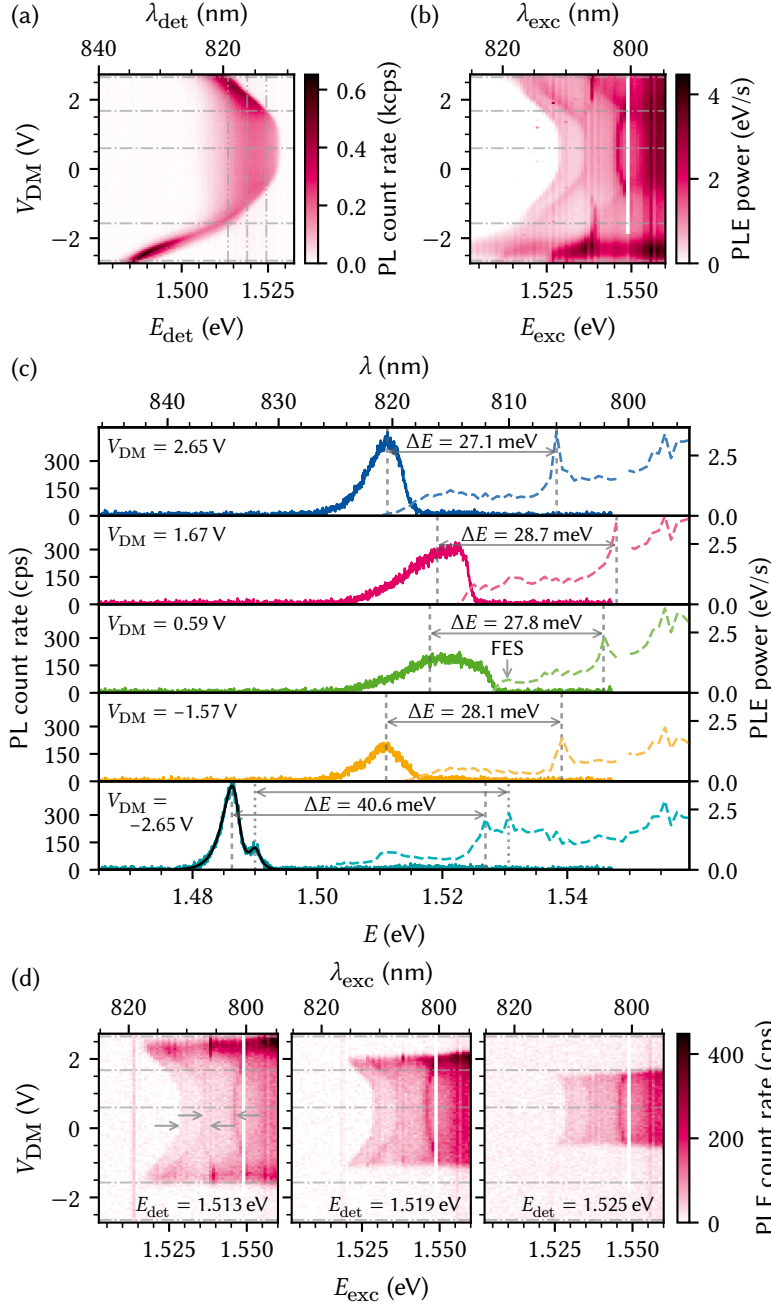
Figure 13.9: Photoluminescence excitation measurement. (a) PL map as function of difference-mode voltage for \lambda_{\text{exc}} = 795 nm (cf. Figure 13.4). (b) PLE map. Each column corresponds to a map like in (a) integrated up to the laser line at E_{\text{det}} = E_{\text{exc}} . While a 2DEG exists ( V_{\text{DM}} \in [-1.6 \text{ V}, 2.6 \text{ V}] ), absorption in PLE sets on just as emission stops in PL at the Fermi edge \mu (see also Figure B.1). The Fermi edge feature is replicated at least once at approximately 10 meV above \mu , while a feature with positive Stark shift \alpha > 0 duplicated at least once as well appears with apexes at E_{\text{exc}} = 1.536 eV and 1.546 eV. A sharp feature appears as the 2DEG is close to depletion at 1.538 eV. The vertical white bar is missing data. (c) Line cuts of the PL (a, solid lines) and PLE maps (b, dashed) taken at the horizontal dash-dotted gray lines there. At V_{\text{DM}} = -2.65 V, the PL line is split by 3.7 meV which is replicated in the PLE spectrum 40.6 meV higher. The black line shows a fit to a trion and exciton following Reference 295. The features at around 1.555 eV do not shift with the voltage and are thus likely unrelated to the trap. (d) Line cuts of the entire data set at single detection energies indicated by vertical dash-dot-dotted lines in (a). Horizontal dash-dotted lines are again the positions of the line cuts shown in (c). Arrows indicate a splitting of approximately 10 meV.
