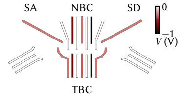
Figure 6.4: Gate layout of a quadruple quantum dot with two charge sensor QDs from Reference 80. Ohmic contacts used for transport measurements are right (left) of SA (SD). NBC and TBC are the gates in the middle of the top and bottom rows. The gates are colored according to the voltages applied with the device hosting a single large QD in the few-electron, sequential tunneling regime.
