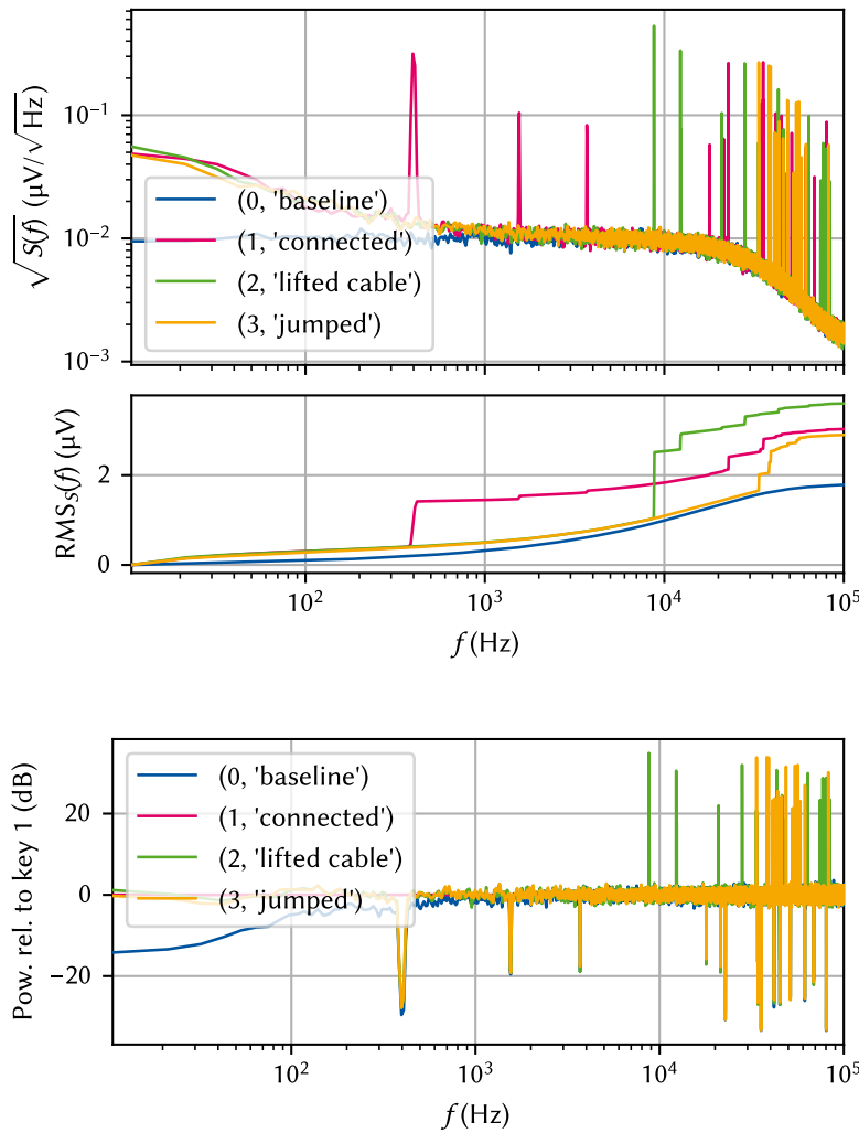
Figure 3.5: The python_spectrometer plot shown in Figure 3.3 when setting spect.plot_cumulative = True . This adds a subplot that shows the RMS (see Equation 2.14) which can be helpful in evaluating the contribution of individual peaks in the spectrum to the total noise power. Both the oscilloscope subplot (Figure 3.4) and the RMS subplot can also be shown at the same time.
