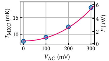
Figure 6.3: Mixing chamber temperature as function of nanositioner AC readout voltage. The secondary axis indicates the conversion from T_{\text{MXC}} to power obtained in Figure 6.2 which is approximately linear in this regime, leading to the expected P \sim R^{-1} V_{\text{AC}}^2 behavior. Solid line is a fit to the power with R = 16.9 \text{ k}\Omega .
