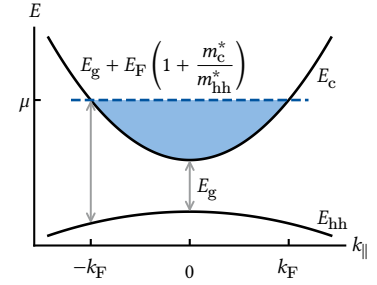
Figure 11.1: Band structure diagram of a doped heterostructure (after Reference 232). Due to the n -type doping, the conduction band is filled up to the Fermi level \mu . Photonic excitation of an electron-hole pair can only occur at |k| > k_F into the free states above \mu due to the small photon momentum. Recombination can occur within a bandwidth of E_F(1 + m_c^*/m_{hh}^*) .
