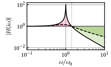
Figure 8.1: Force transmission function of a damped harmonic oscillator with \gamma = \omega_0/200 (solid black line) and \gamma = \omega_0/2 (dashed black line). Below the break frequency \omega = \sqrt{2}\omega_0 (dotted vertical line), external excitations are amplified (shaded red area). For larger damping \gamma , the amplification at resonance becomes smaller. Above \omega = \sqrt{2}\omega_0 , excitations are attenuated (shaded green area). Both amplification below and attenuation above the break frequency become smaller as the damping rate \gamma is increased.
