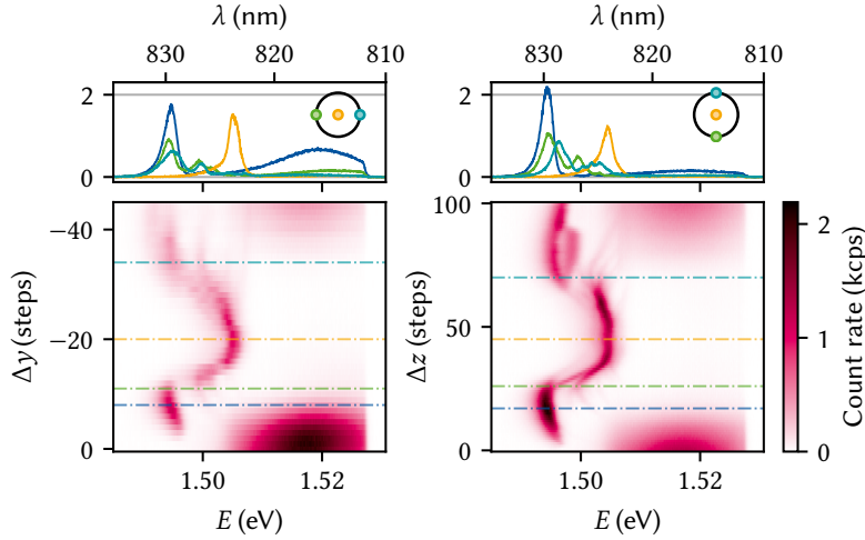
Figure 13.8: PL of a large exciton trap as function of position perpendicular (left) and parallel (right) to gravity. The trap is biased so that the emission is Stark-shifted towards lower energy. Upper panels show line cuts taken along the dash-dotted lines in the lower panels, demonstrating fairly identical behavior along both axes. The cuts in orange, green, and teal are taken at the positions indicated on the circle in the upper panel representing the trap gate.
