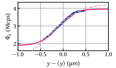
Figure A.1: Reflectance gradient of the edge of a Au gate electrode on the bare GaAs surface. The dashed line is a fit to Equation 8.8 with \mathcal{R}_0 fixed while the solid includes this parameter in the fit.
