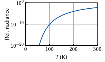
Figure 6.1: Relative black-body radiance obtained by integrating Equation 6.1 from \lambda = 0 \mu\text{m} to 4.5 \mu\text{m} and normalizing to the total radiance. At T = 300 K, the fraction of total radiance residing in the high-energy part of the spectrum is still only 0.6 %.
