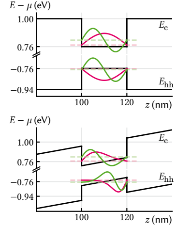
Figure 11.3: QCSE in an undoped QW. Top: conduction and heavy-hole valence band profiles along the growth direction. The wave functions of the first two eigenstates in the well are drawn in magenta and green, respectively. The ground state transition is larger by \Delta E = 17 \text{ meV} than the gap E_g due to the confinement. Bottom: same structure as above with an out-of-plane electric field applied across the structure ( F = 5 \text{ V}/\mu\text{m} ). Analytical wave functions in the infinite-well approximation are shown in magenta and green again. The wave functions get pushed to opposite interfaces of the QW, lowering the ground state transition energy by \Delta E = -10 \text{ meV} . Excitonic effects are not included.
