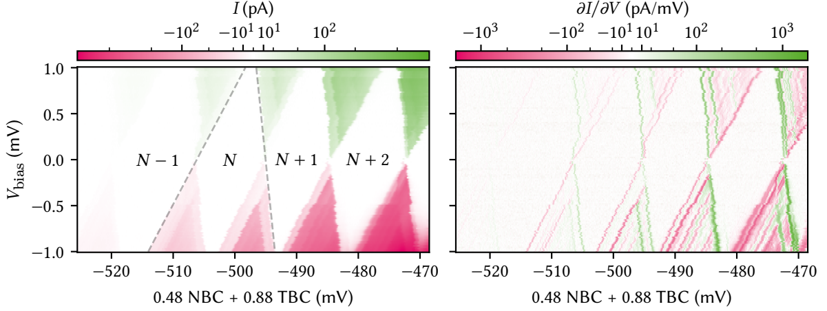
Figure 6.5: Coulomb diamond measurement of the single GDQD confined by applying static voltages to the gates shown in Figure 6.4. The left panel shows the current measured with a transimpedance amplifier (TIA) with a bias applied on one side of the device. The horizontal axis shows the virtual plunger gate swept for each bias voltage indicated on the vertical axis. The difference in slope of the dashed gray lines around the N -electron diamond yields the lever arm \alpha converting virtual plunger gate voltage to (relative) energy inside the dot. From the fact that the slopes are not equal up to a sign we can infer that the coupling to source and drain reservoirs is unequal also, indicating that either the dot is situated closer to SA than to SD, or the topology of the tunneling contacts in the 2DEG is different due to different electrostatic potential. The right panel shows the differential conductance obtained from differentiating the data from the left panel along the plunger gate axis. Clearly visible are several additional transition lines which correspond to excited states inside the dot becoming energetically available within the bias window.
