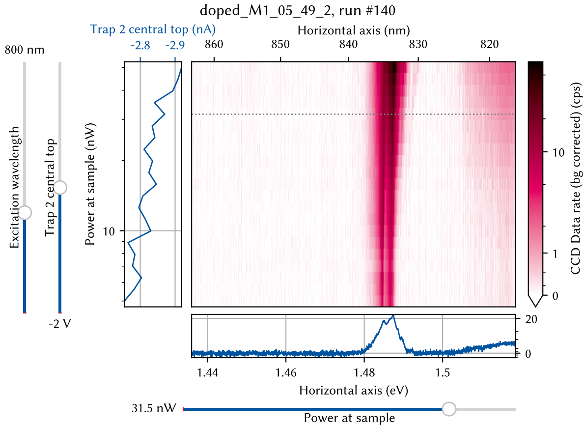
Figure 12.4: The plot_nd() plot window. The bottom panel, enabled by default, shows a horizontal line cut through the 2D data of the main panel whose y-value can be set with the adjacent slider widget. The left panel shows the leakage currents of gates that participate in the sweep and, if measured, the laser power. A vertical slider widget is added for each data dimension not displayed on the x or y axis of the main plot. The figure title shows the sample as well as the measurement identifiers assigned by QCoDeS.
