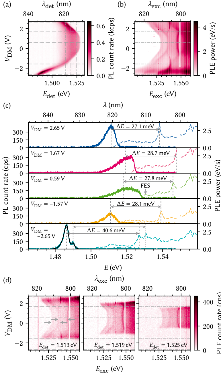
Figure 13.9: Photoluminescence excitation measurement. (a) PL map as function of difference-mode voltage for \lambda_{exc} = 795 nm (cf. Figure 13.4). (b) PLE map. Each column corresponds to a map like in (a) integrated up to the laser line at E_{det} = E_{exc} . While a 2DEG exists ( V_{DM} \in [-1.6 V, 2.6 V]), absorption in PLE sets on just as emission stops in PL at the Fermi edge \mu (see also Figure B.1). The Fermi edge feature is replicated at least once at approximately 10 meV above \mu , while a feature with positive Stark shift \alpha > 0 duplicated at least once as well appears with apexes at E_{exc} = 1.536 eV and 1.546 eV. A sharp feature appears as the 2DEG is close to depletion at 1.538 eV. The vertical white bar is missing data. (c) Line cuts of the PL (a, solid lines) and PLE maps (b, dashed) taken at the horizontal dash-dotted gray lines there. At V_{DM} = -2.65 V, the PL line is split by 3.7 meV which is replicated in the PLE spectrum 40.6 meV higher. The black line shows a fit to a trion and exciton following Reference 295. The features at around 1.555 eV do not shift with the voltage and are thus likely unrelated to the trap. (d) Line cuts of the entire data set at single detection energies indicated by vertical dash-dot-dotted lines in (a). Horizontal dash-dotted lines are again the positions of the line cuts shown in (c). Arrows indicate a splitting of approximately 10 meV.
