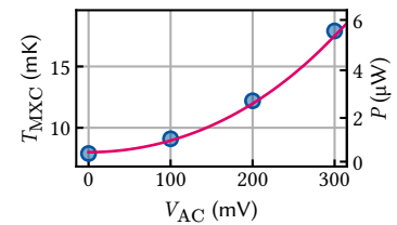
Figure 6.3: Mixing chamber temperature as function of nanopositioner AC readout voltage. The secondary axis indicates the conversion from T_{\text{MXC}} to power obtained in Figure 6.2 which is approximately linear in this regime, leading to the expected P \sim R^{-1} V_{\text{AC}}^2 behavior. Solid line is a fit to the power with R = 16.9 \text{ k}\Omega .
