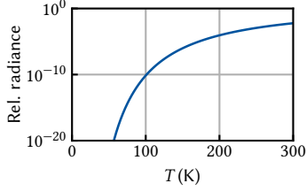
Figure 6.1: Relative black-body radiance obtained by integrating Equation 6.1 from \lambda = 0 \mu\text{m} to 4.5 \mu\text{m} and normalizing to the total radiance. At T = 300 \text{ K} , the fraction of total radiance residing in the high-energy part of the spectrum is still only 0.6 %.
