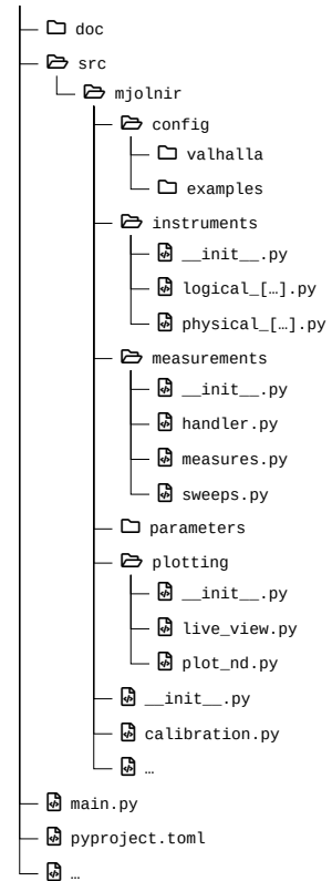
Figure 12.2: Source tree structure of the mjoInir package. Logical QCoDeS instruments and parameters are defined in the instruments and parameters modules, respectively. Instruments are configured using yaml files located in a config subdirectory. The measurements module provides classes for the abstraction of measurements using QCoDeS underneath. Live plots of instrument data as well as a plot function for multidimensional measurement data are defined in the plotting module. calibration.py contains routines for power, CCD, and excitation rejection calibrations. The main.py file is a code cell-based script that serves as the entrypoint for measurements.
