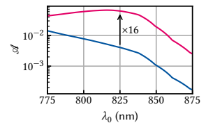
Figure 13.10: QW absorbance \mathcal{A} in a heterostructure with default (blue) and optimized (magenta) barrier thickness and top and bottom gates as function of wavelength. Optimization was performed at 825 nm using the differential evolution algorithm implemented in PyMoosh, resulting in a barrier thickness of 122 nm and an absorbance better by a factor of 16 at 6.3 %.
