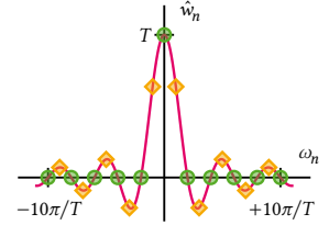
Figure 2.3: The Fourier representation of the rectangular window in continuous time (solid line) and for discrete frequencies \omega_n = 2\pi n/T (circles). Introducing a phase shift, that is, shifting the window with respect to the signal in time, effectively shifts \omega_n \rightarrow \omega_n + \eta as indicated for \eta = 1/2 (diamonds). This incurs scalping loss.
