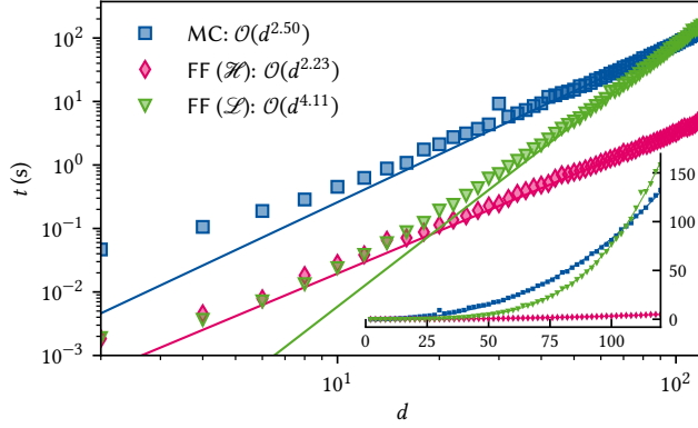
Figure 16.2: Performance of the formalism using Equation 16.36 compared to a Monte Carlo method for a single gate as a function of problem dimension d . Parameters are: n_M = 1, n_\alpha = 3, n_{MC} = 100, f_{UV} = 10^2/\Delta t, n_\omega = 500 where n_\alpha is the number of noise operators considered, n_{MC} the number of Monte Carlo trajectories over which is averaged, and n_\omega the number of frequency samples. The calculation using filter functions clearly outperforms MC for small system sizes. For dimensions larger than d \approx 100 (roughly equivalent to 7 qubits) Monte Carlo (blue squares) performs better than the FF calculation with transfer matrices (green triangles) for this set of parameters and processor due to the better scaling behavior. Using conjugation by unitaries (orange diamonds) significantly outperforms MC also for large dimensions. While the fits to t = ad^b (lines) underestimate the leading order exponent due to the data not being in the asymptotic regime, they support the expected relationship of complexity between the approaches. The inset shows the same data on a linear scale, highlighting the different scaling behaviors for large d .
