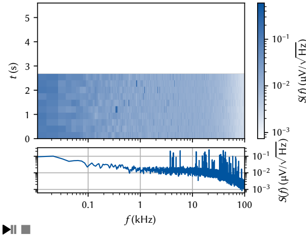
Figure 3.8: Spectrometer live view. The bottom plot shows the most recently acquired spectrum, while the top plot shows a waterfall plot of the most recent ones. Data acquisition runs in a background thread, keeping the interpreter responsive and available to interact with instruments, for example. The icons in the bottom left and right corners allow interacting with the live view.
