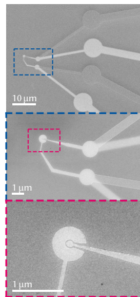
Figure 13.1: SEM image of an exciton trap with both central and guard gates. Gates on the bottom side are visible through the membrane. Images taken by Thomas Descamps.
