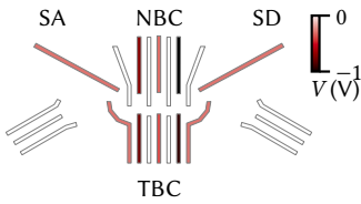
Figure 6.4: Gate layout of a quadruple quantum dot with two charge sensor QDs from Reference 80. Ohmic contacts used for transport measurements are right (left) of SA (SD). NBC and TBC are the gates in the middle of the top and bottom rows. The gates are colored according to the voltages applied with the device hosting a single large QD in the few-electron, sequential tunneling regime.
