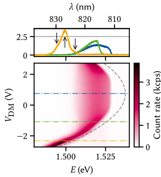
Figure 13.4: PL as function of difference-mode voltage on a large exciton trap. The observed Stark shift follows roughly the expected quadratic dispersion, but is offset by 0.75 V with respect to zero bias. Dashed gray line is a guide to the eye of a parabola with curvature -3.5 \text{ meV/V}^2 . Line cuts in the upper panel are taken at the voltages indicated by dash-dotted lines in the lower, and arrows indicate positions of individual peaks making up the yellow line shape.
