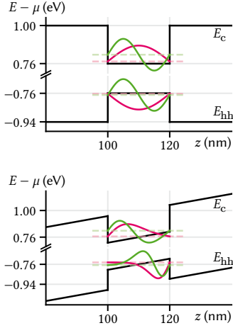
Figure 11.3: QCSE in an undoped QW. Top: conduction and heavy-hole valence band profiles along the growth direction. The wave functions of the first two eigenstates in the well are drawn in magenta and green, respectively. The ground state transition is larger by \Delta E = 17 \text{ meV} than the gap E_g due to the confinement. Bottom: same structure as above with an out-of-plane electric field applied across the structure ( F = 5 \text{ V}/\mu\text{m} ). Analytical wave functions in the infinite-well approximation are shown in magenta and green again. The wave functions get pushed to opposite interfaces of the QW, lowering the ground state transition energy by \Delta E = -10 \text{ meV} . Excitonic effects are not included.
