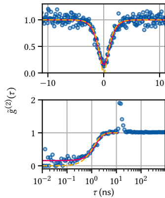
Figure 7.9: g^{(2)} measurement of the emission line at 872.267 nm under cw excitation with 1 \mu\text{W} at 793 nm. The monochromator bandwidth was \Delta\lambda = 200 \text{ pm} = 325 \mu\text{eV} .
