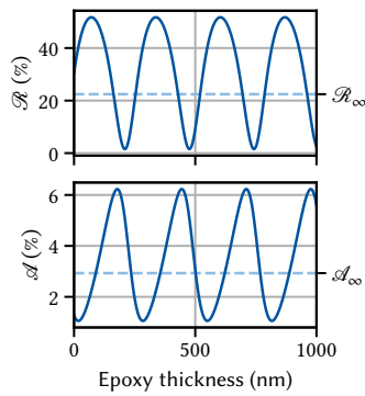
Figure B.3: Reflectance (top) and QW absorptance (bottom) as function of epoxy thickness assuming coherent back-scattering. The period corresponds to the wavelength in epoxy, \lambda_{\text{epo}} = \lambda_0 / n_{\text{epo}} .
