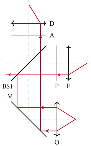
Figure 9.1: Reduced sketch of the optical path (cf. Figure 7.1) including the cold mirror (M). The excitation laser experiences four reflections, twice at M and once each at the sample and at BS1. The light emitted from the sample experiences a single reflection at M.
