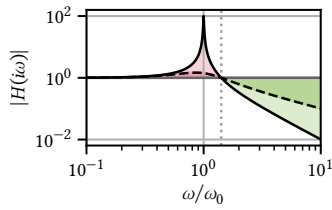
Figure 8.1: Force transmission function of a damped harmonic oscillator with \gamma = \omega_0/100 (solid black line) and \gamma = \omega_0/2 (dashed black line). Below the break frequency \omega = \sqrt{2}\omega_0 (dotted vertical line), external excitations are amplified (shaded red area). For larger damping \gamma , the amplification at resonance becomes smaller. Above \omega = \sqrt{2}\omega_0 , excitations are attenuated (shaded green area). Both amplification below and attenuation above the break frequency become smaller as the damping rate \gamma is increased.
