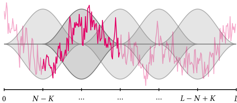
Figure 2.5: Illustration of Welch's method for spectrum estimation. The data (magenta) of length L is partitioned into K = 2L/N - 1 segments of length N . Each segment is multiplied by a window function (gray) which reduces spectral leakage and other artifacts. A finite overlap K between adjacent windows (gray) ensures efficient sample use.
