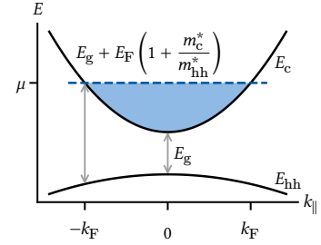
Figure 11.1: Band structure diagram of a doped heterostructure (after Reference 232). Due to the n -type doping, the conduction band is filled up to the Fermi level \mu . Photonic excitation of an electron-hole pair can only occur at |k| > k_F into the free states above \mu due to the small photon momentum. Recombination can occur within a bandwidth of E_F(1 + m_c^*/m_{hh}^*) .
