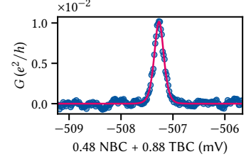
Figure 6.6: Conductance of a Coulomb resonance in the sequential tunneling regime. The magenta line is a fit to Equation 6.8 with T = 74.9 \text{ mK} and \Gamma = 0.524(5) \mu\text{eV} .
