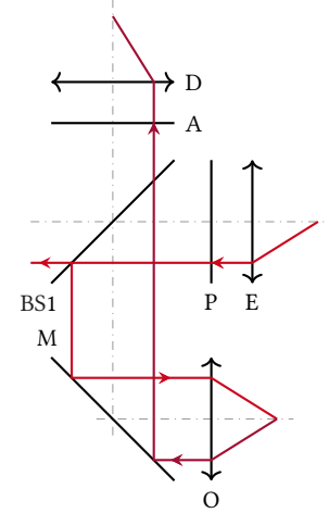
Figure 9.1: Reduced sketch of the optical path ( cf. Figure 7.1) including the cold mirror (M). The excitation laser experiences four reflections, twice at M and once each at the sample and at BS1. The light emitted from the sample experiences a single reflection at M.
