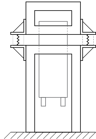
Figure 8.2: Sketch of the cryostat suspension. There are two separate frames (thick black lines), the upper of which the cryostat (grey outline) is attached to. The frames are connected by air springs mounted on angle brackets extruding from the frames.
