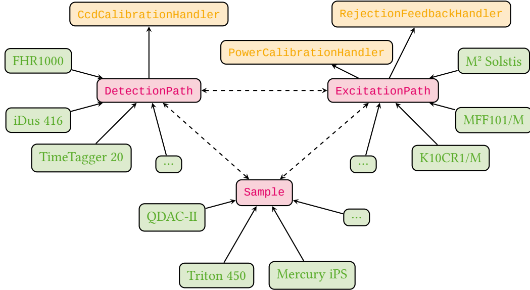
Figure 12.1: Abstraction of physical instruments. mjoInir defines three logical instrument classes (magenta) that represent different aspects of the experiment and group various physical instruments (green). Logical instruments expose various logical parameters that include communication with multiple physical instruments. Sample can be subclassed to suit the particular type of device under investigation. Calibration handlers (orange) are controlled by the logical instruments governing the optical path. Logical instruments are part of a QCoDeS Station and can interact with each other as indicated by the dashed arrows.
