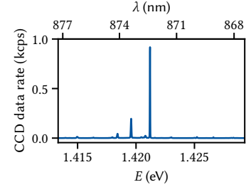
Figure 7.8: PL spectrum of a SAQD under cw excitation at 793 nm.
