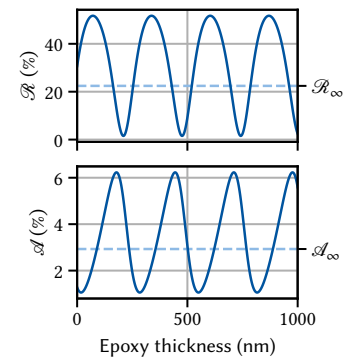
Figure B.3: Reflectance (top) and QW absorptance (bottom) as function of epoxy thickness assuming coherent back-scattering. The period corresponds to the wavelength in epoxy, \lambda_{\text{epo}} = \lambda_0 / n_{\text{epo}} .
