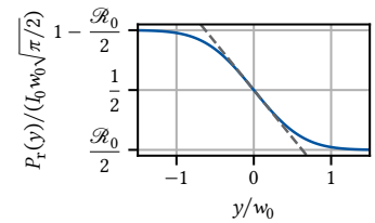
Figure 8.5: Theoretical reflected power for a Gaussian beam of width w_0 and a reflectance contrast of 1 - \mathcal{R}_0 according to Equation 8.8. The dashed line indicates the leading order approximation at y = 0 .
