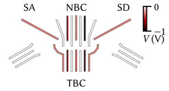
Figure 6.4: Gate layout of a quadruple quantum dot with two charge sensor QDs from Reference 80. Ohmic contacts used for transport measurements are right (left) of SA (SD). NBC and TBC are the gates in the middle of the top and bottom rows. The gates are colored according to the voltages applied with the device hosting a single large QD in the few-electron, sequential tunneling regime.
