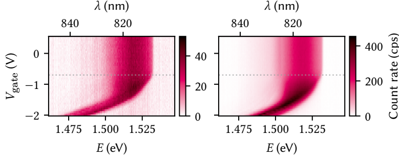
Figure 13.3: PL as function of gate voltage on a single fan-out gate on the bottom (left) and top (right) side of the membrane. The behavior is qualitatively similar but the overall quantum efficiency lower by an order of magnitude for gates on the bottom (as-grown buried) side. Dotted gray lines are a guide to the eye demonstrating that the changes to the PL spectrum set in at the same voltage for both types of gates (around -0.7 V).
