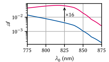
Figure 13.10: QW absorptance \mathcal{A} in a heterostructure with default (blue) and optimized (magenta) barrier thickness and top and bottom gates as function of wavelength. Optimization was performed at 825 nm using the differential evolution algorithm implemented in PyMoosh, resulting in a barrier thickness of 122 nm and an absorptance better by a factor of 16 at 6.3 %.
