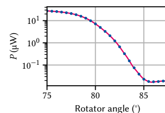
Figure 12.3: Power calibration using the continuously variable ND filter. Error bars from statistics are too small to see. Magenta line is a quadratic smoothing spline.
