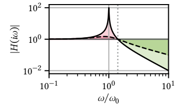
Figure 8.1: Force transmission function of a damped harmonic oscillator with \gamma = \omega_0/100 (solid black line) and \gamma = \omega_0/2 (dashed black line). Below the break frequency \omega = \sqrt{2}\omega_0 (dotted vertical line), external excitations are amplified (shaded red area). For larger damping \gamma , the amplification at resonance becomes smaller. Above \omega = \sqrt{2}\omega_0 , excitations are attenuated (shaded green area). Both amplification below and attenuation above the break frequency become smaller as the damping rate \gamma is increased.
