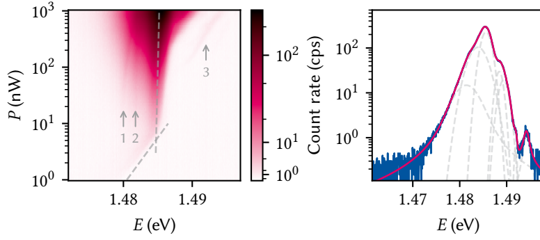
Figure 13.5: PL as function of excitation power P . In the left panel two qualitatively different regimes are indicated by dashed gray lines as guides to the eye; below 10 nW, the main peak displays a blue shift logarithmic in excitation power, E = 1.485 \text{ eV} + 5 \text{ meV} \log_{10} P . Above, the blue shift diminishes significantly. Three additional lines, indicated by arrows, with varying power dispersion are visible. Right panel shows a fit to data at P = 1 \mu\text{W} . A sum of seven individual lines (dashed, gray) is required to fit the data. The dashed gray lines are the individual contributions.
