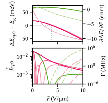
Figure 11.5: Electric field dependence of the QCSE for the first two energy levels in the QW. Top: the ground state energy (magenta) shows the expected quadratic dependence; the confinement energy is compensated at around F = 3.7 V/ \mu\text{m} . Higher in-plane orbital levels ( p ) are shown for the QW ground state in decreasing saturation. For zero field, the splitting is zero as there is no in-plane confinement. At maximum field, the splitting is 2\hbar\omega = 2 meV. Dashed lines (right axis) show the derivative, revealing that the QW excited state is actually raised in energy at low fields. Bottom: oscillator strengths (same color code as above). Dashed lines (right axis) show the electron tunneling rate through the barrier, dash-dotted the holes.
