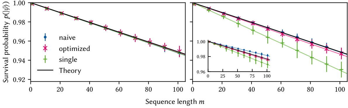
Figure 19.3: Simulation of a RB experiment using 100 random sequences per point for different gate and noise types (see the main text for an explanation of the gate type monikers). Dashed lines are fits of Equation 19.3 to the data while the solid black lines correspond to a zeroth-order RB model with A = B = 0.5 and the true average gate infidelity per Clifford r . Errorbars show the standard deviation of the RB sequence fidelities, illustrating that for the “single” gate set noise correlations can lead to amplified destructive and constructive interference of errors. The same noise spectrum is used for all three error channels ( \sigma_x , \sigma_y , \sigma_z ) and the large plots show the sum of all contributions. (a) Uncorrelated white noise with the noise power adjusted for each gate type so that the average error per gate r is constant over all gate types. No notable deviation is seen between different gate types. (b) Correlated 1/f -like noise with noise power adjusted to match the average Clifford fidelity in (a). The decay of the “single” gate set differs considerably from that of the other gate sets and the RB decay expected for the given average gate fidelity, whereas “naive” and “optimized” gates match the zeroth order RB model well, indicating that correlations in the noise affect the relation between RB decay and average gate fidelity in a gate-set-dependent way. Inset: contributions from \sigma_z -noise show that the sequence fidelity can be better than expected for certain gate types and noise channels.
