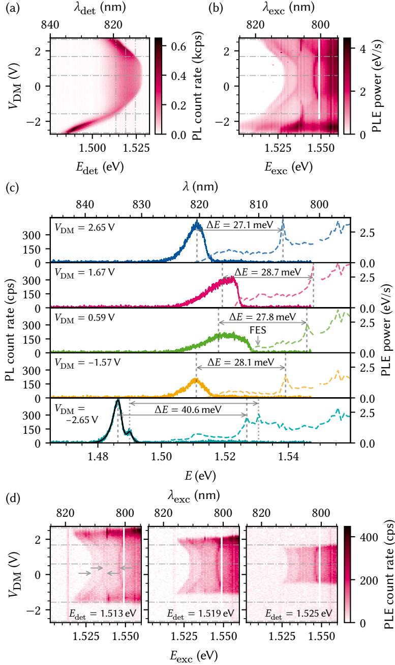
Figure 13.9: Photoluminescence excitation measurement. (a) PL map as function of difference-mode voltage for \lambda_{exc} = 795 nm (cf. Figure 13.4). (b) PLE map. Each column corresponds to a map like in (a) integrated up to the laser line at E_{det} = E_{exc} . While a 2DEG exists ( V_{DM} \in [-1.6 \text{ V}, 2.6 \text{ V}] ), absorption in PLE sets on just as emission stops in PL at the Fermi edge \mu (see also Figure B.1). The Fermi edge feature is replicated at least once at approximately 10 meV above \mu , while a feature with positive Stark shift \alpha > 0 duplicated at least once as well appears with apexes at E_{exc} = 1.536 eV and 1.546 eV. A sharp feature appears as the 2DEG is close to depletion at 1.538 eV. The vertical white bar is missing data. (c) Line cuts of the PL (a, solid lines) and PLE maps (b, dashed) taken at the horizontal dash-dotted gray lines there. At V_{DM} = -2.65 V, the PL line is split by 3.7 meV which is replicated in the PLE spectrum 40.6 meV higher. The black line shows a fit to a trion and exciton following Reference 295. The features at around 1.555 eV do not shift with the voltage and are thus likely unrelated to the trap. (d) Line cuts of the entire data set at single detection energies indicated by vertical dash-dot-dotted lines in (a). Horizontal dash-dotted lines are again the positions of the line cuts shown in (c). Arrows indicate a splitting of approximately 10 meV.
