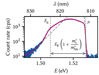
Figure 13.2: PL of the bare 2DEG. Magenta line is a smoothing spline fit to the data. Indicated by dotted gray lines are the Fermi edge at high and the band edge at low energy. The Fermi edge has a Fermi distribution (exponential indicated by a dashed gray line) whose temperature is typically much higher than the lattice temperature ( \sim 1 K). Below the band edge there is an exponential tail (dashed gray line) due to impurities that permeates far into the gap.
