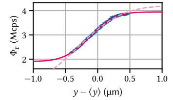
Figure A.1: Reflectance gradient of the edge of a Au gate electrode on the bare GaAs surface. The dashed line is a fit to Equation 8.8 with \mathcal{R}_0 fixed while the solid includes this parameter in the fit.
