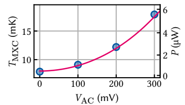
Figure 6.3: Mixing chamber temperature as function of nanositioner AC readout voltage. The secondary axis indicates the conversion from T_{\text{MXC}} to power obtained in Figure 6.2 which is approximately linear in this regime, leading to the expected P \sim R^{-1} V_{\text{AC}}^2 behavior. Solid line is a fit to the power with R = 16.9 \text{ k}\Omega .
