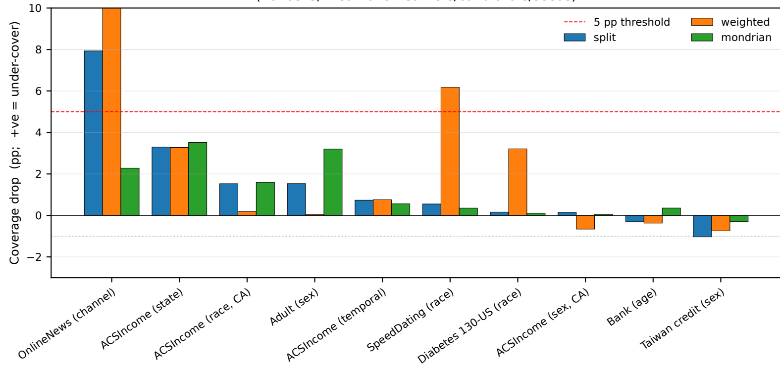
Worst-OOD coverage drop per task, by CP variant (10 tasks, mean over learners/calibrators/seeds)
