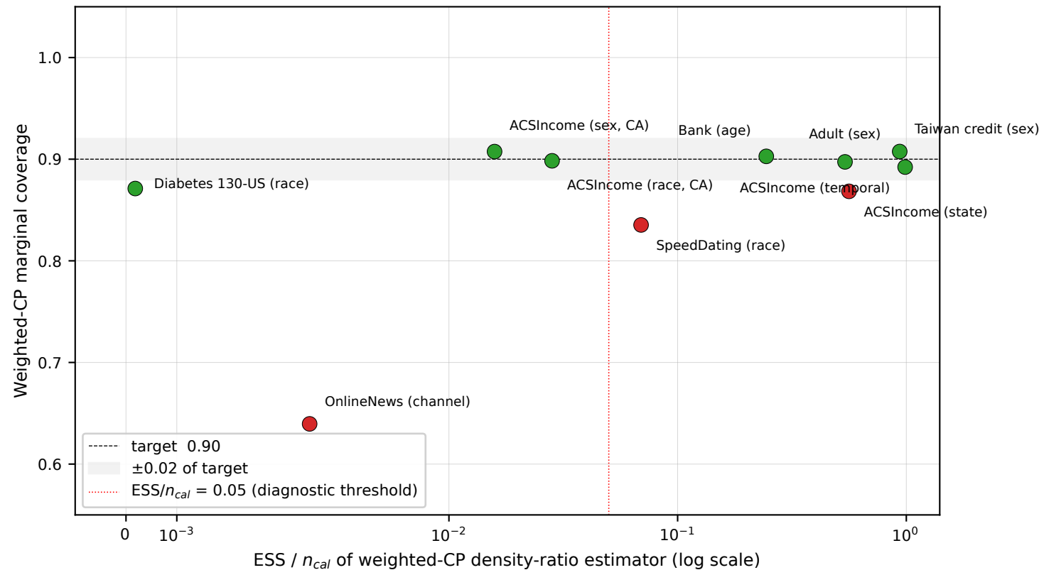
Weighted-CP coverage vs density-ratio ESS (10-task panel; one point per task)
