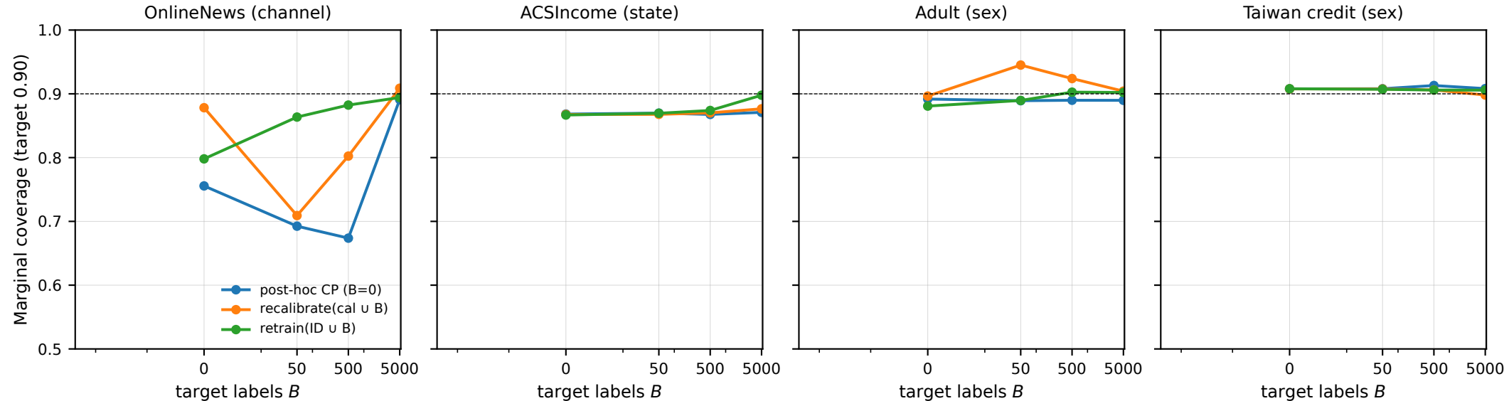
Budget-axis: marginal coverage vs target-label budget, 4 representative tasks (HGB, 3 seeds)
