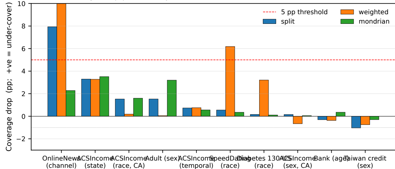
Worst-OOD coverage drop per task, by CP variant (10 tasks, mean over learners/calibrators/seeds)
