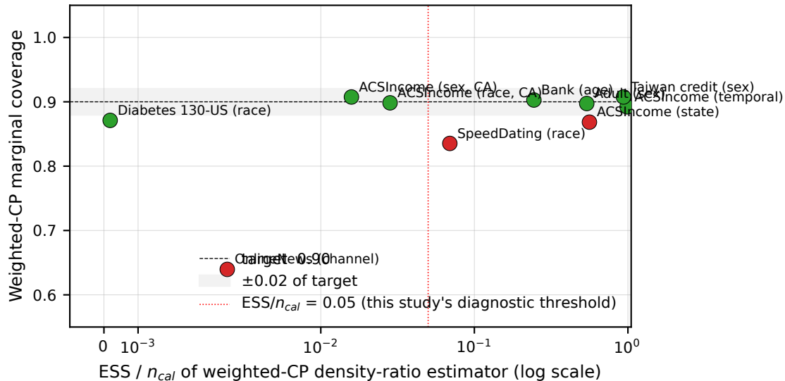
Weighted-CP coverage vs density-ratio ESS (10-task panel; one point per task)
