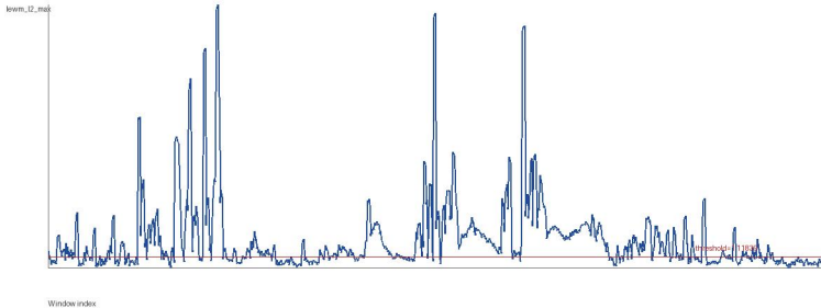
Latent surprise trajectory: Shooting Error (buggy)
