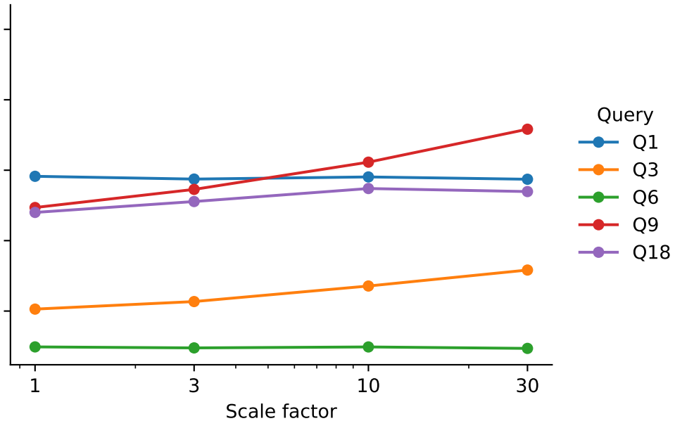
Tectorwise
