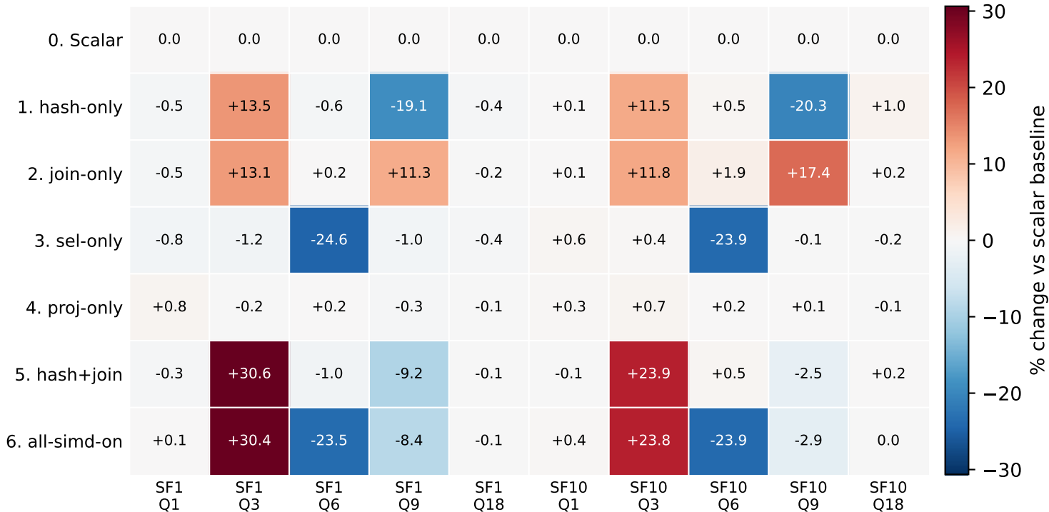
SIMD ablation: cycles change vs scalar baseline
