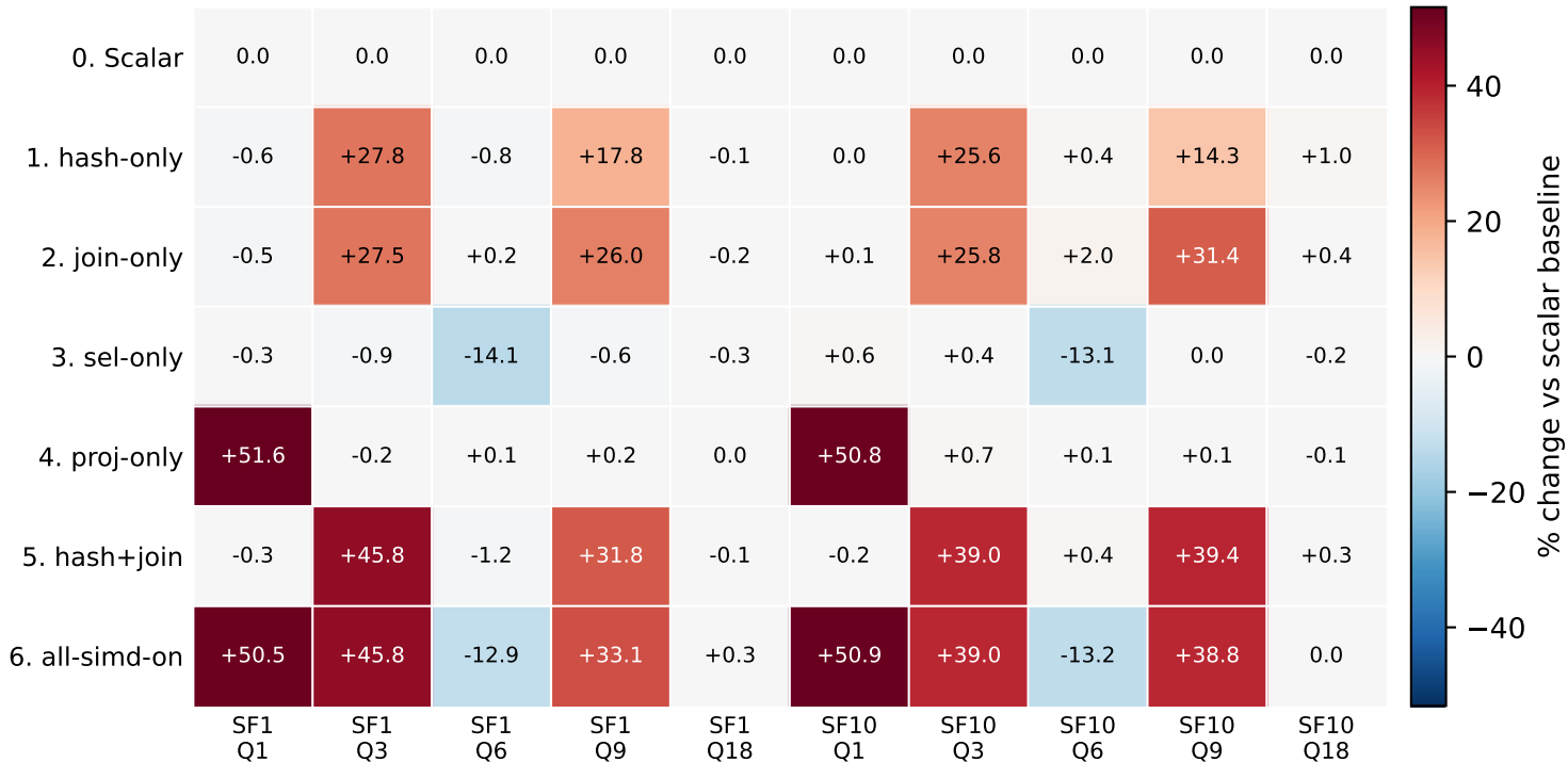
SIMD ablation: time change vs scalar baseline
