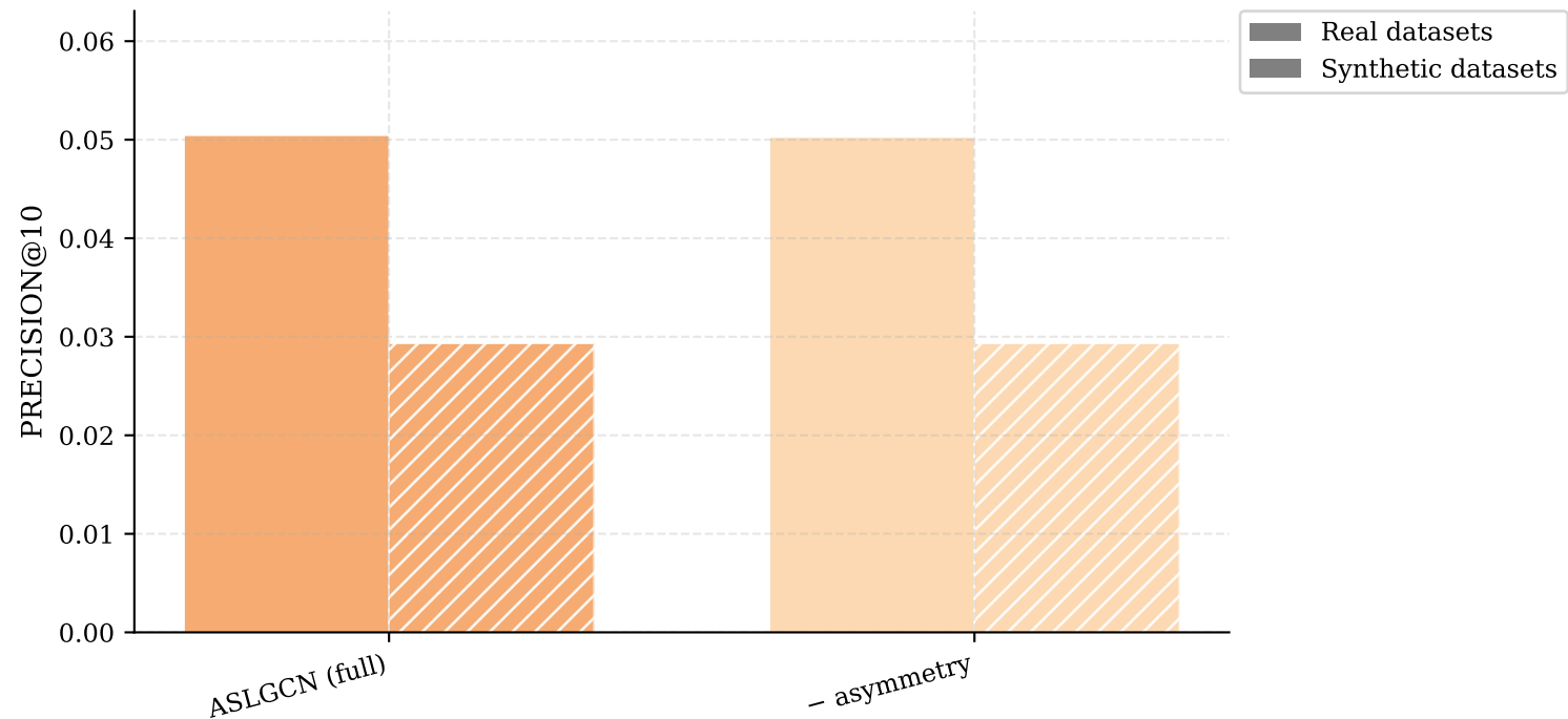
ASLGCN Ablations — PRECISION@10
