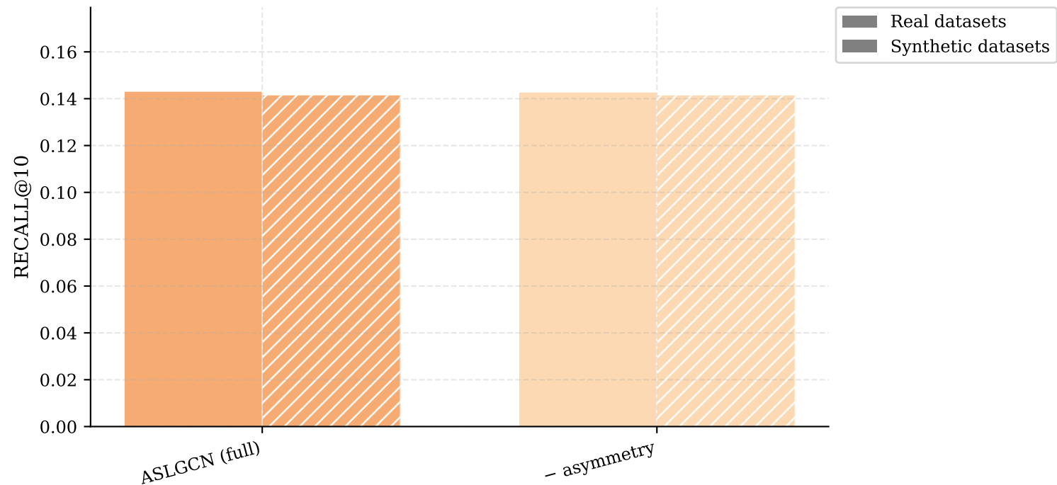
ASLGCN Ablations — RECALL@10
