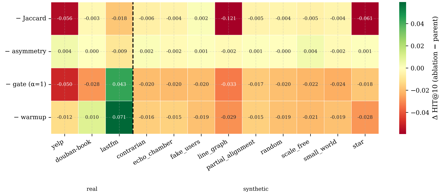
Ablation Impact: \Delta HIT@10 vs. Parent Model
