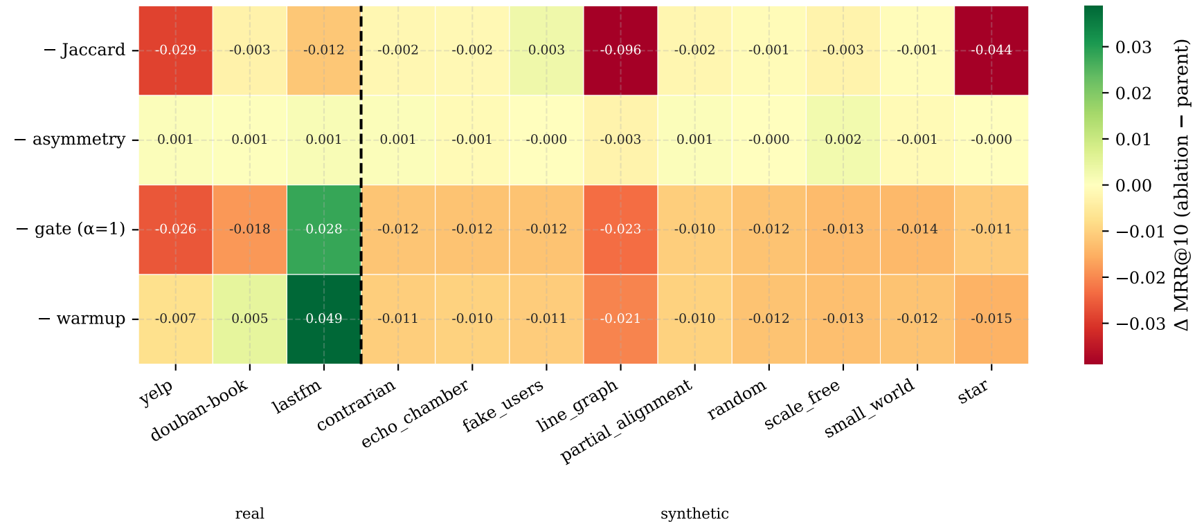
Ablation Impact: \Delta MRR@10 vs. Parent Model
