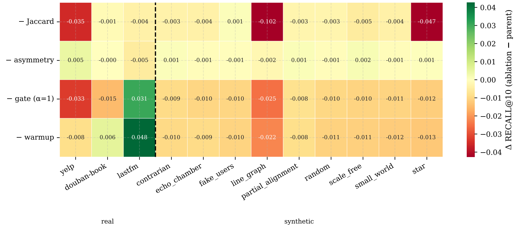
Ablation Impact: \Delta RECALL@10 vs. Parent Model
