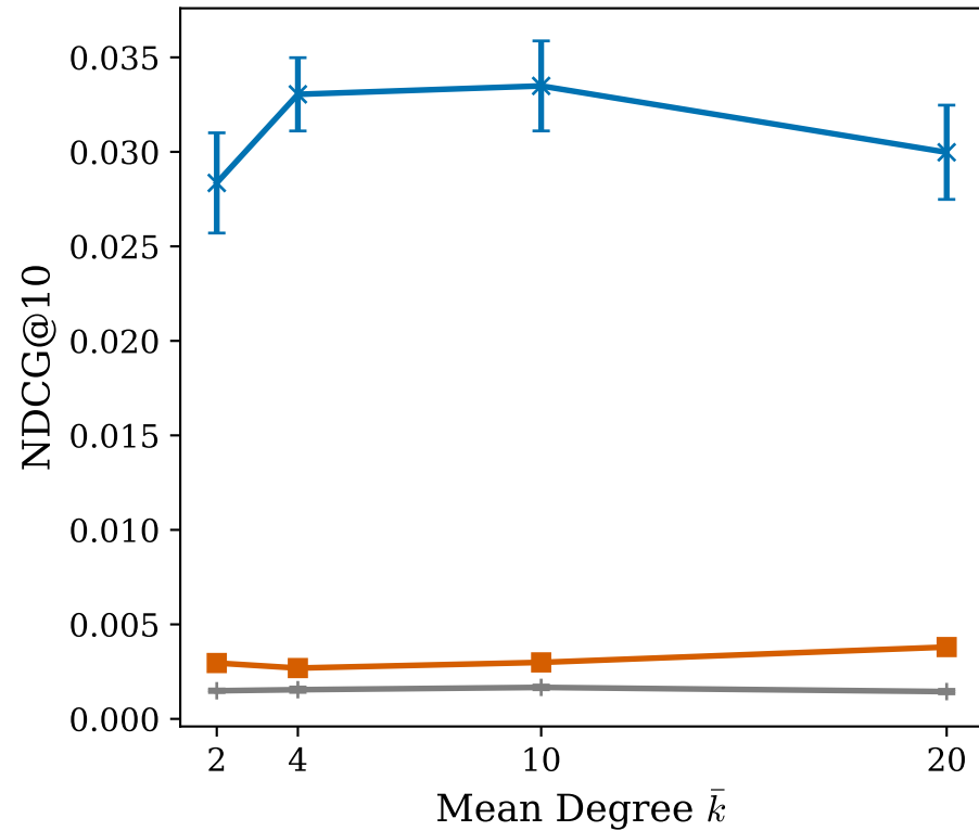
Echo Chamber
