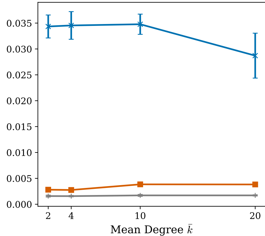
Contrarian
