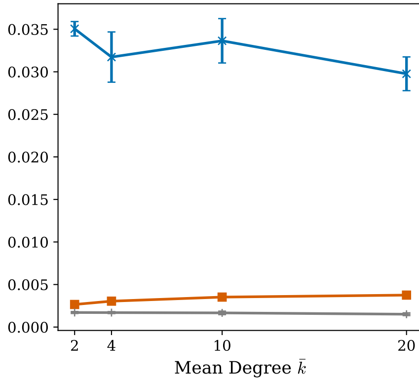
Partial Alignment
