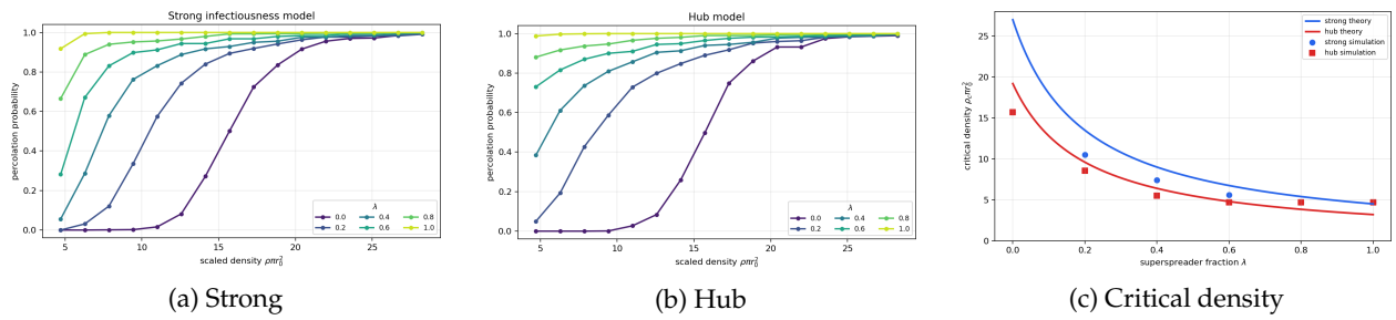
Figure 1: Percolation probability and critical density. Increasing \lambda shifts the percolation transition to lower density; the hub model has a lower critical density because long-range contacts connect distant clusters more efficiently.
