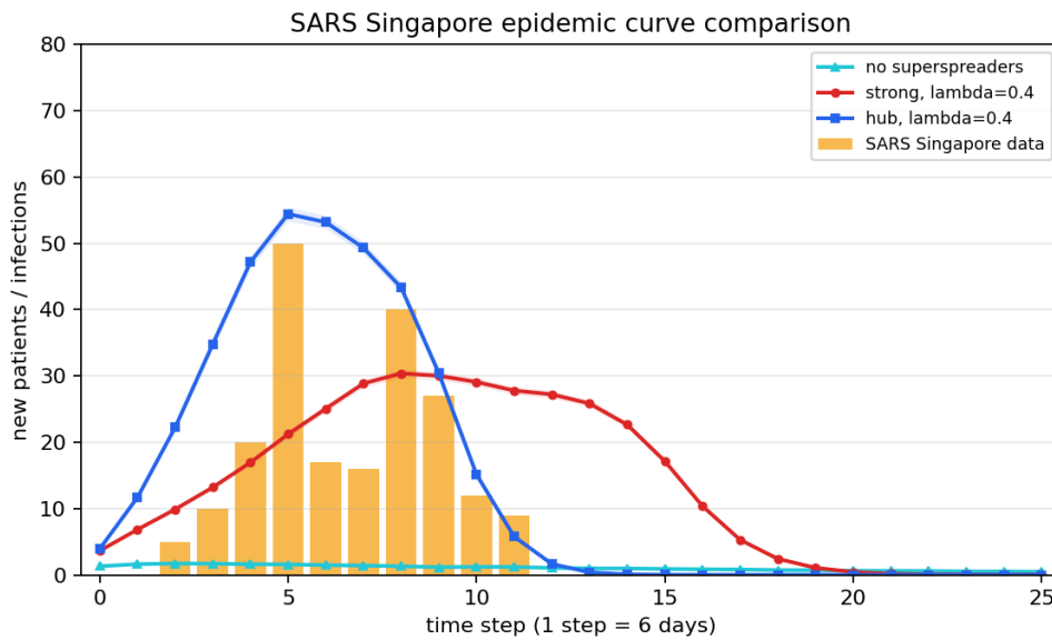
Figure 4: Comparison with the SARS Singapore epidemic curve. The orange bars are six-day binned SARS data digitized from the reference figure. The simulated curves are averages over 1000 Monte Carlo runs using N = 477 , \rho\pi r_0^2 = 15.0 , \lambda = 0.4 for the two superspreader models, and \gamma = 1.0 . The comparison is qualitative, following the role of Fig. 15 in the reference paper.
