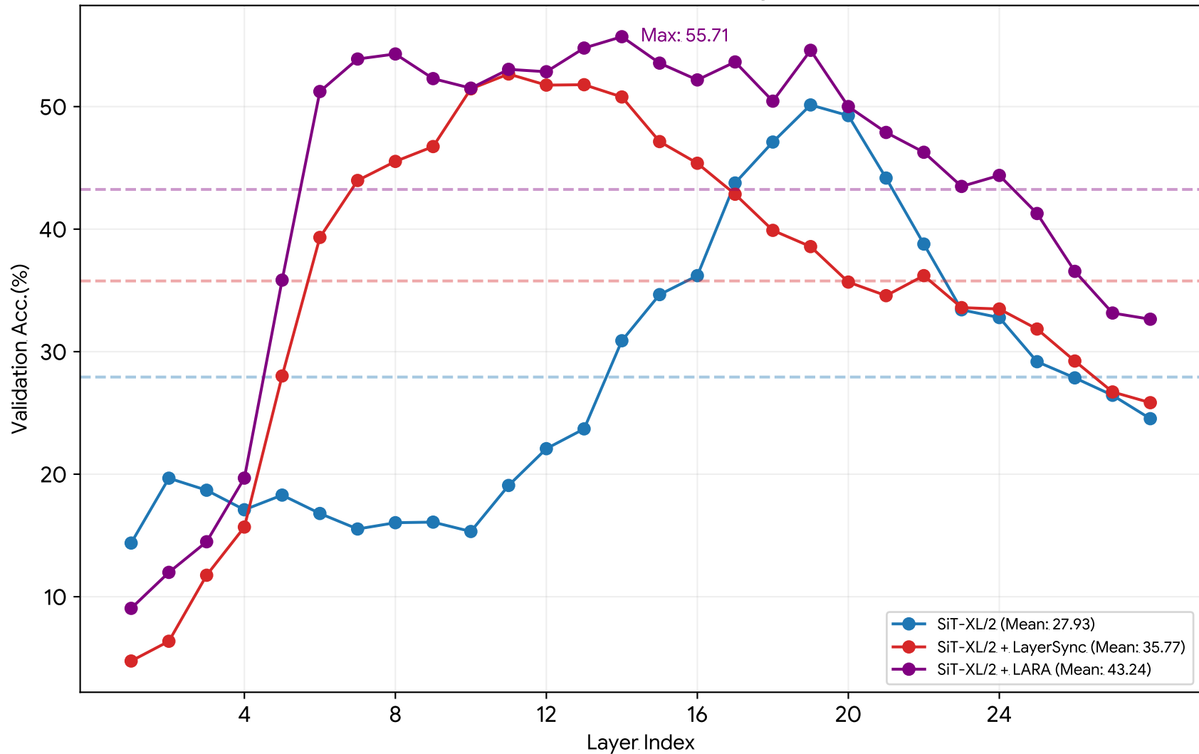
Classification on Tiny ImageNet
