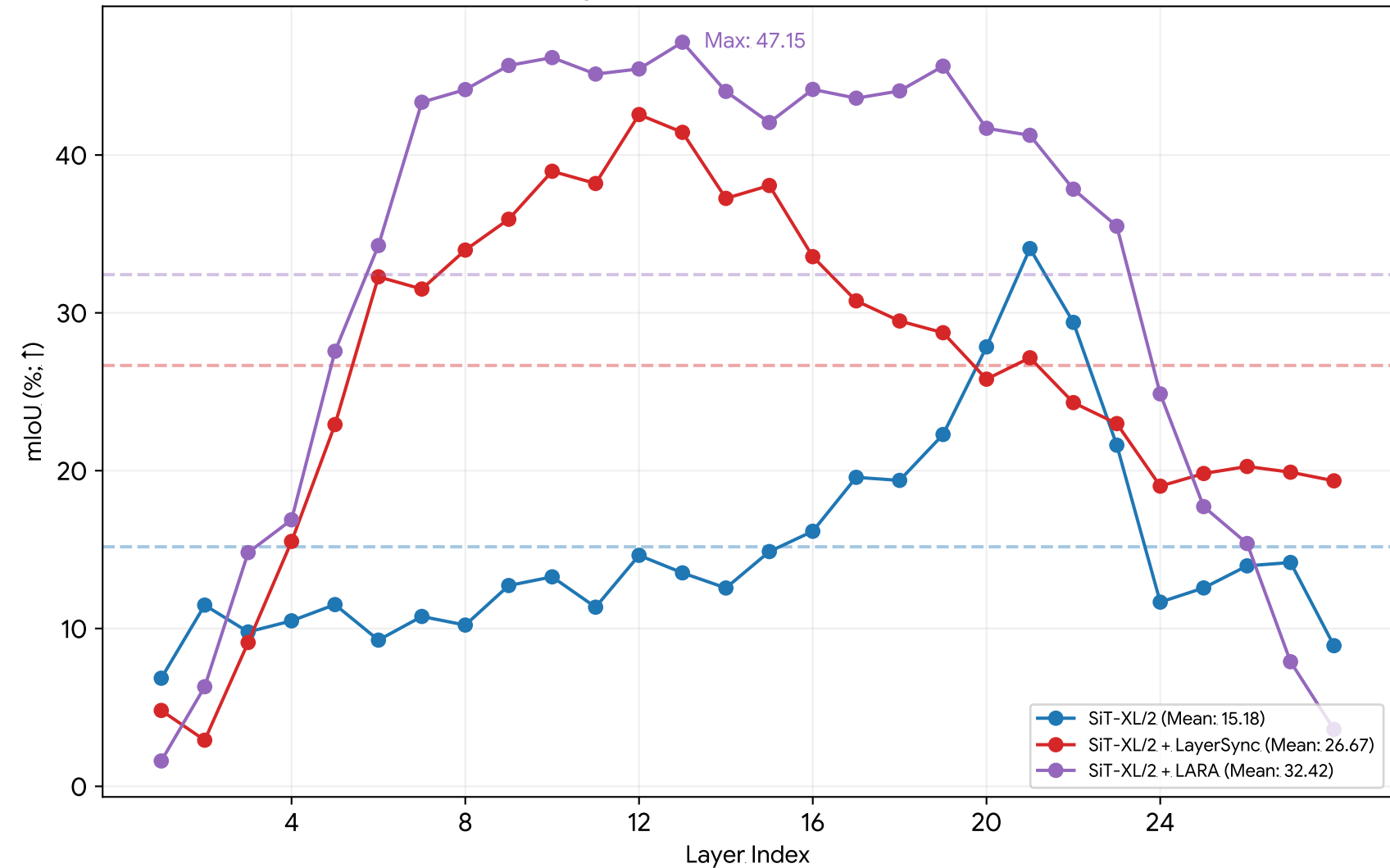
Semantic Segmentation on PASCAL VOC dataset
