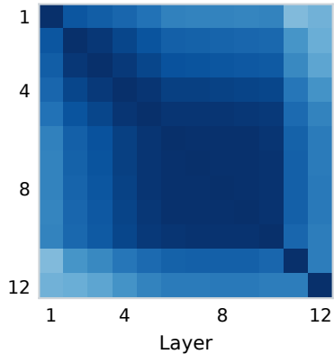
(a) 0x diversity weight No diversity loss
