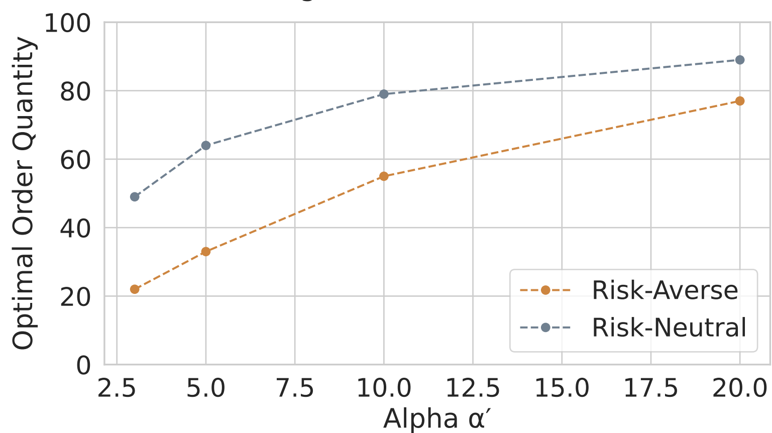
OOQ for right-skewed beta distributions
