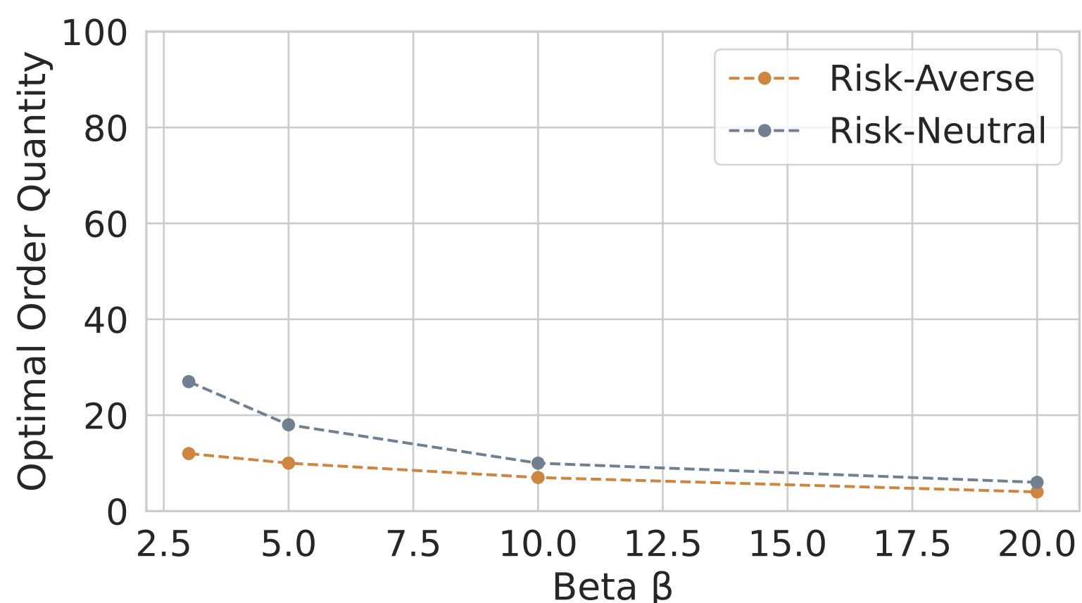
OOQ for right-skewed beta distributions
