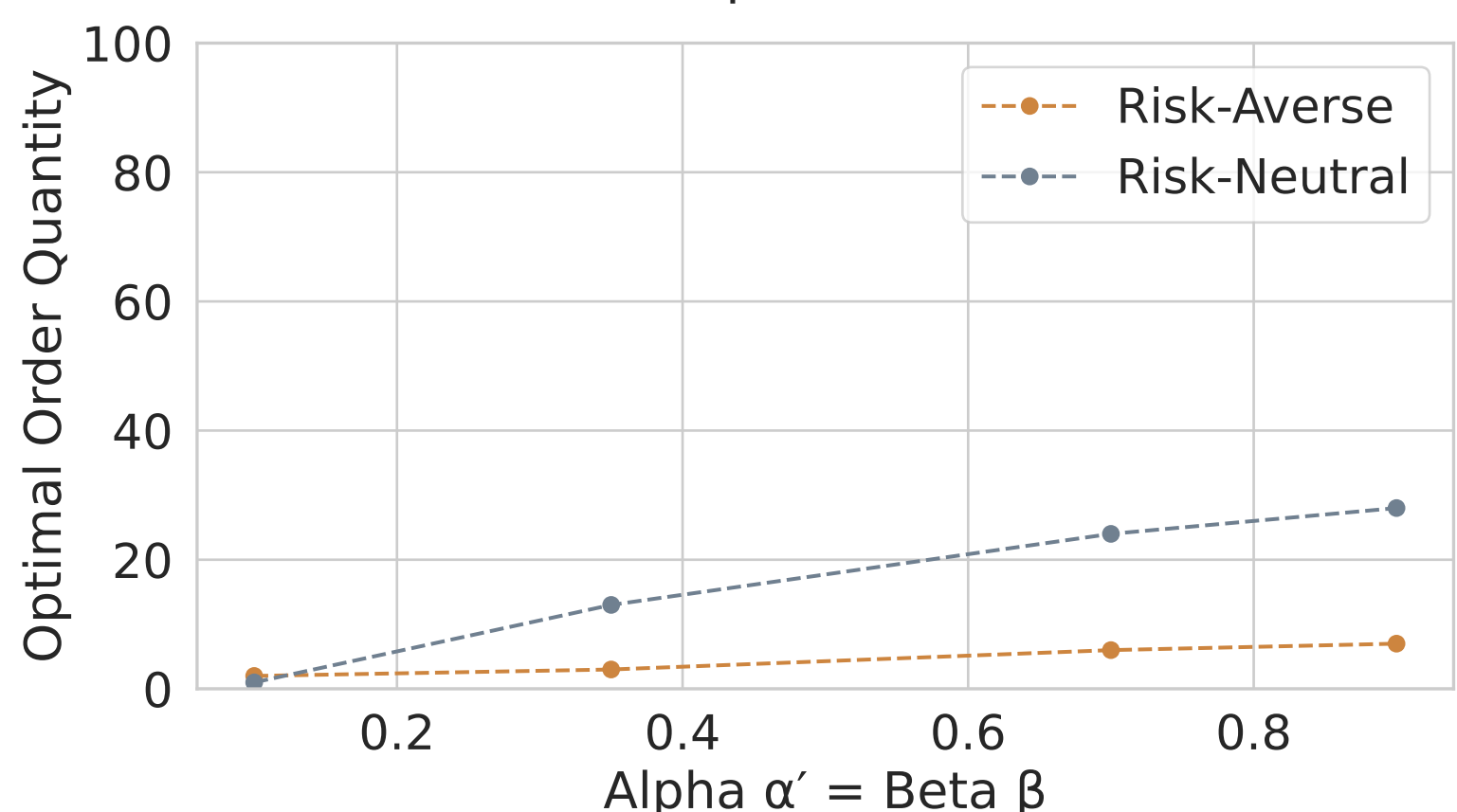
OOQ for left-skewed beta distributions
