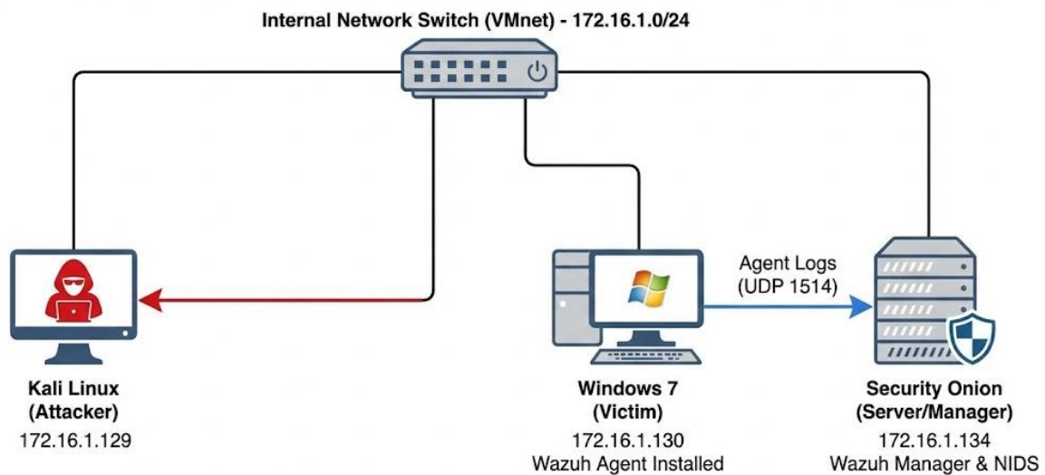
Network Security Monitoring Lab Topology
