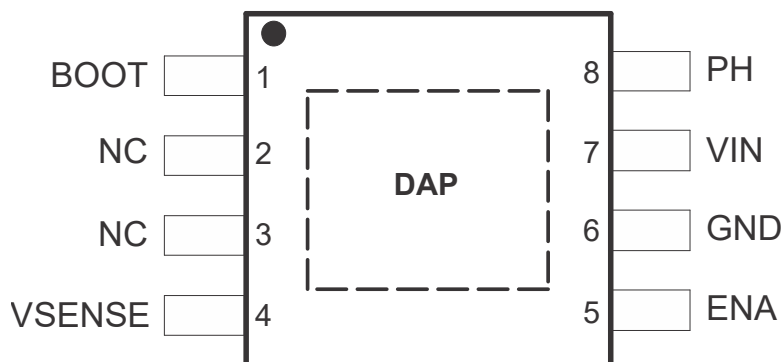
Figure 4-1. DDA Package 8-Pin HSOIC With Thermal Pad (Top View)
