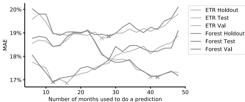
Figure 18.4: Results with a holdout dataset.
