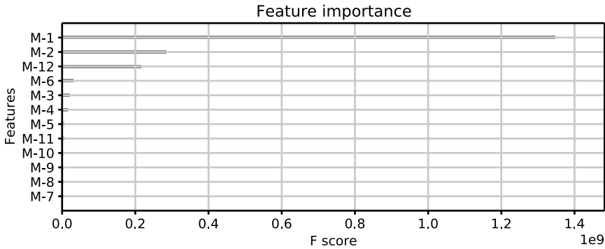
Figure 21.1: XGBoost feature importance.
