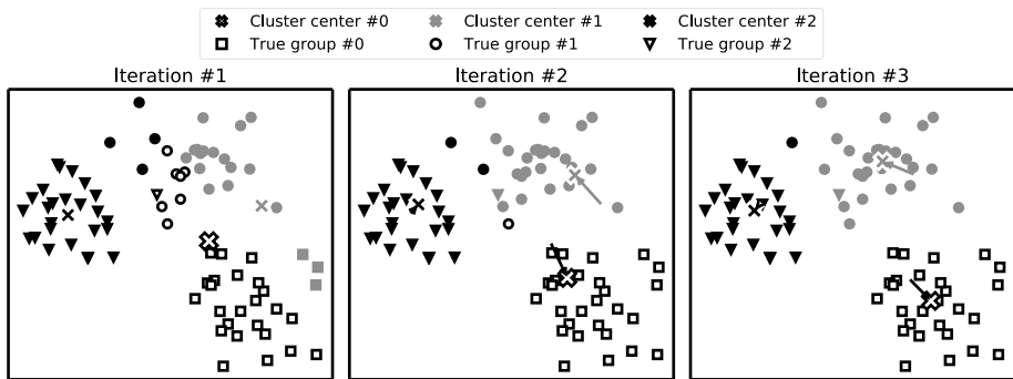
Figure 23.1: K-means with three centers.
