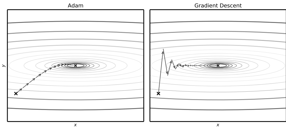
Figure 25.9: Comparison of Adam and gradient descent going through a valley (Adam in 32 steps, gradient descent in 89).
