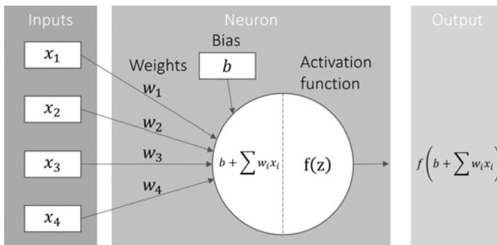
Figure 25.1: Artificial neuron with four inputs.
