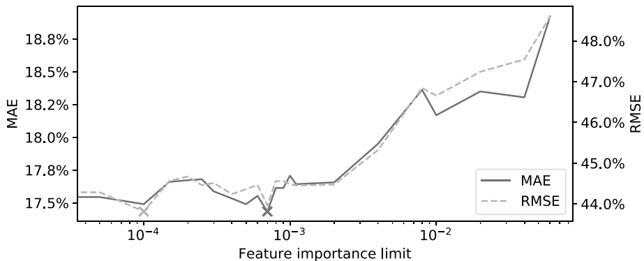
Figure 24.1: Impact of feature selection on the validation set.
