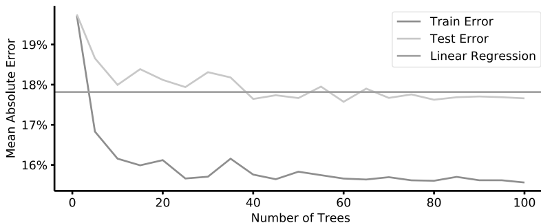
Figure 17.1: Impact of the number of trees for the extremely randomized trees model.
