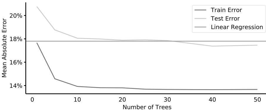
Figure 15.1: Accuracy based on number of trees.
