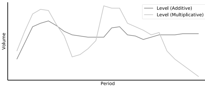
Figure 11.2: Level estimation.
