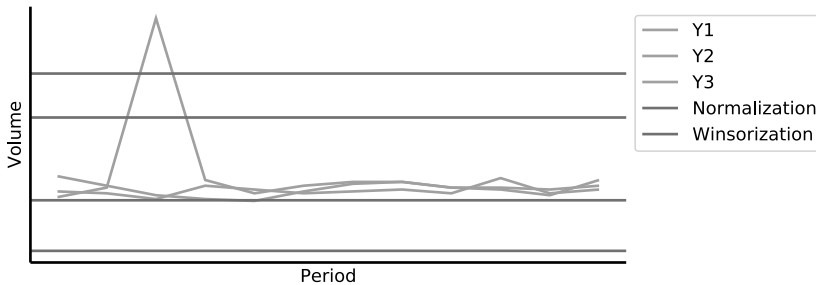
Figure 10.5: Extreme dataset.
