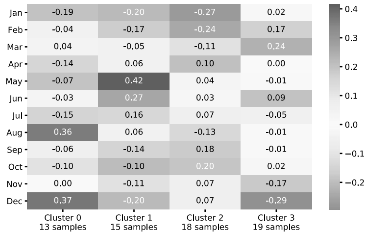
Figure 23.4: Scaled clusters.
