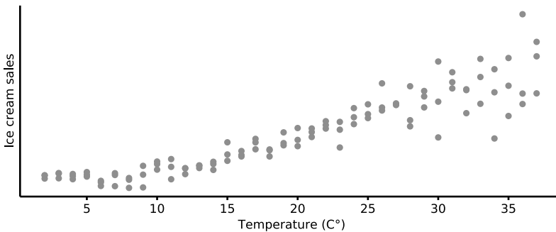
Figure 20.3: “My sales are not so linearly correlated to temperature.”
