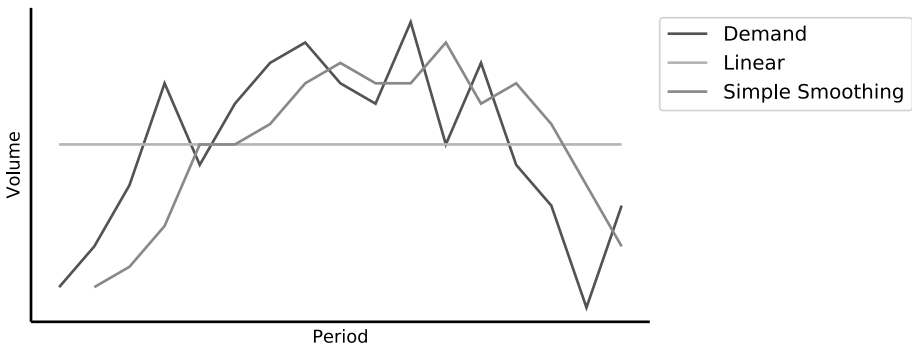
Figure 4.1: Linear regression vs. simple smoothing.
