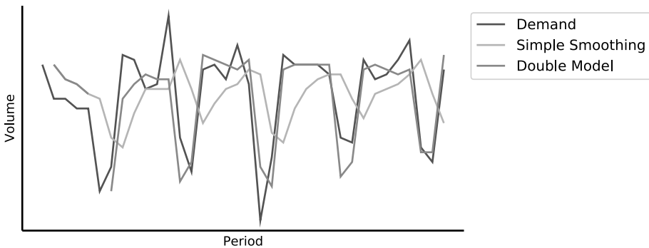
Figure 4.3: Double model vs. simple smoothing.
