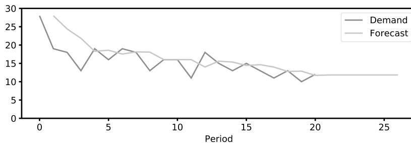
Figure 6.6: Best model selected by our optimization function.
