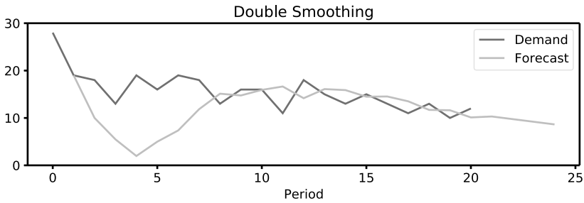
Figure 5.7: Example of double smoothing forecast.
