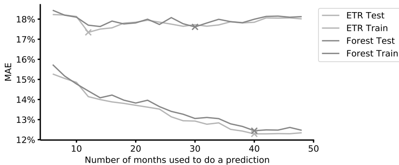
Figure 18.2: Feature optimization.
