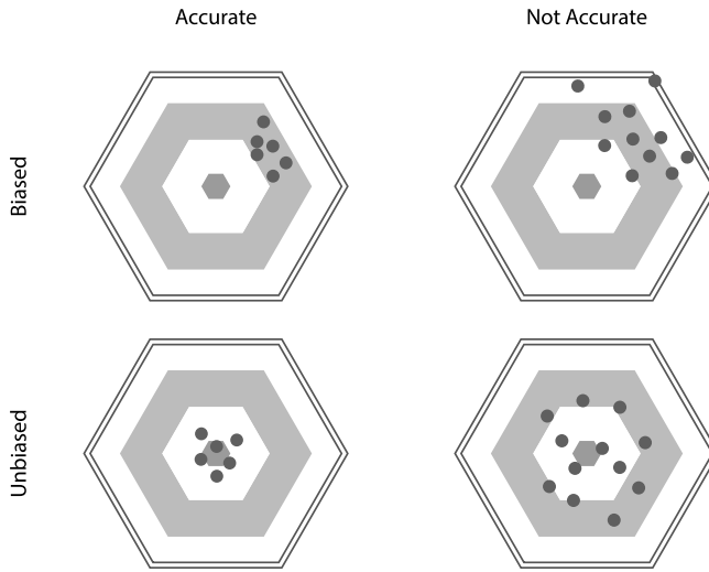
Figure 2.1: Accuracy and bias.
