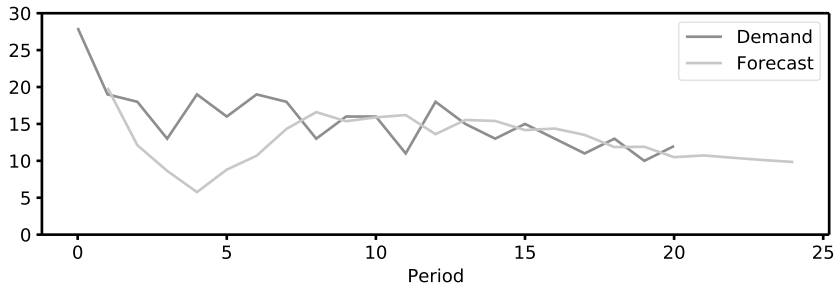
Figure 7.4: Damped double smoothing.
