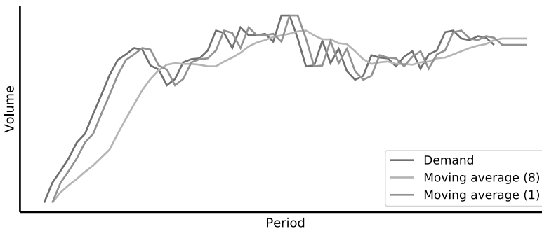
Figure 1.1: Moving averages.
