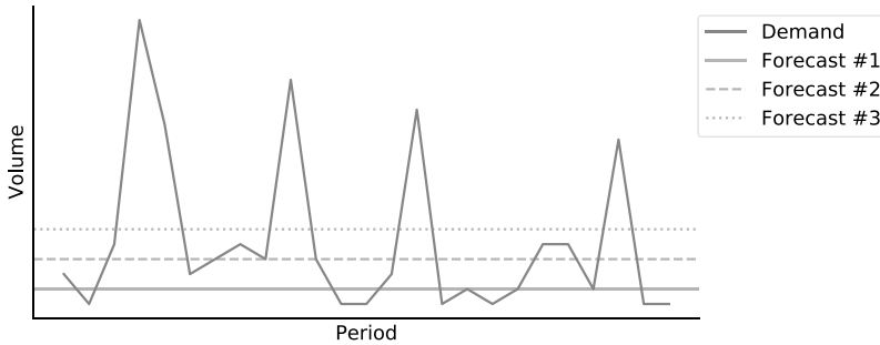
Figure 2.6: Demand and forecasts.
