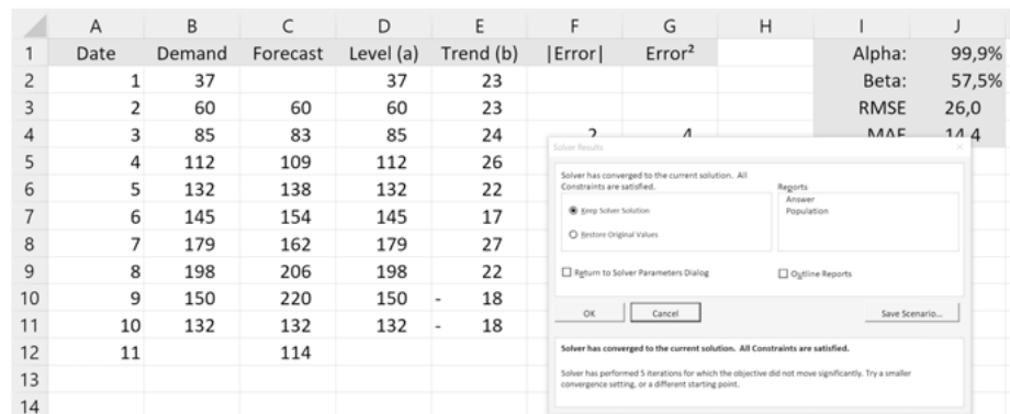
Figure 6.5: Optimization results.
