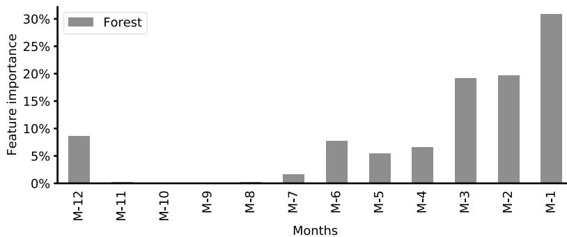
Figure 16.1: Feature importance.
