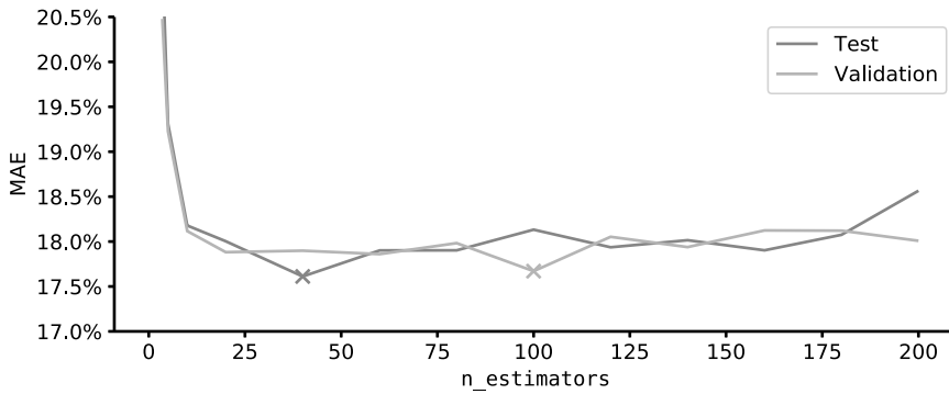
Figure 19.3: Adaboost vs. test set (with learning_rate=0.25 , max_depth=8 , loss='linear' ).
