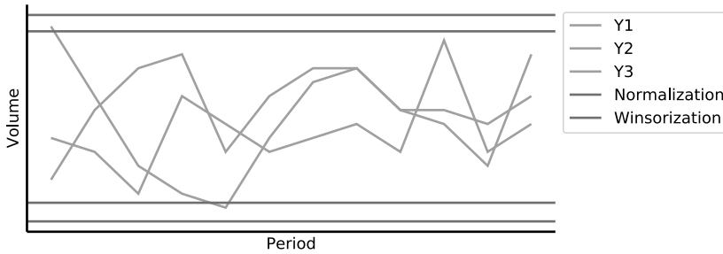
Figure 10.4: Simple dataset.
