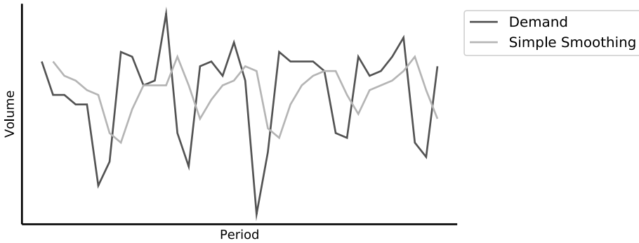
Figure 4.2: Example of simple smoothing applied to ice cream sales.
