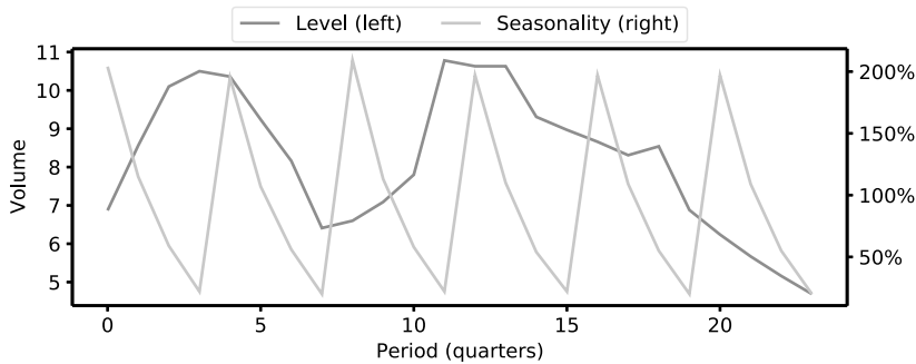
Figure 9.5: Level and seasonality evolution.
