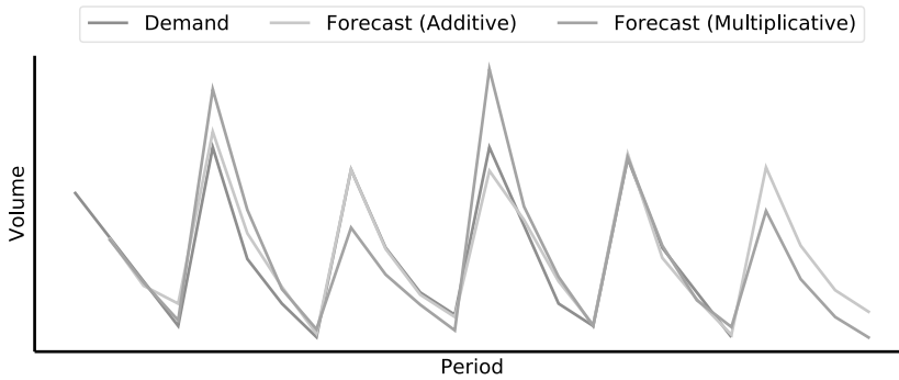
Figure 11.1: Additive forecast.
