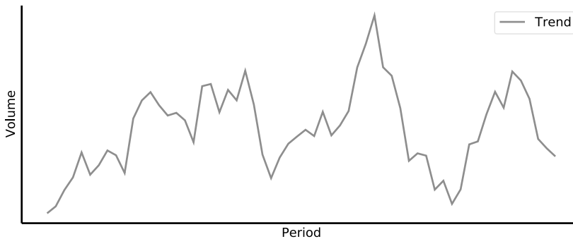
Figure 9.3: Trend.
