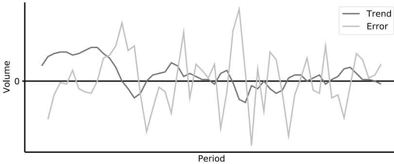
Figure 5.2: Trend and error.
