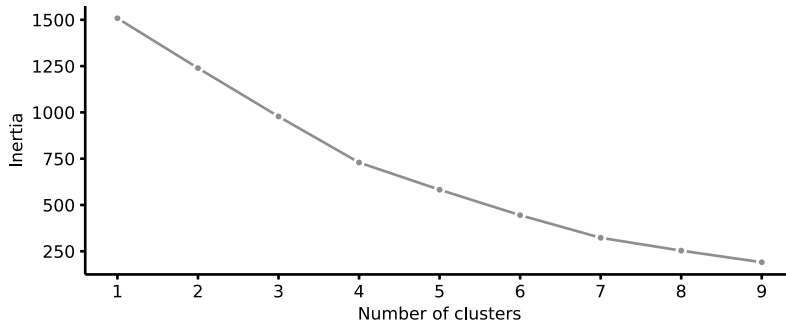
Figure 23.2: Impact of the number of clusters on inertia.
