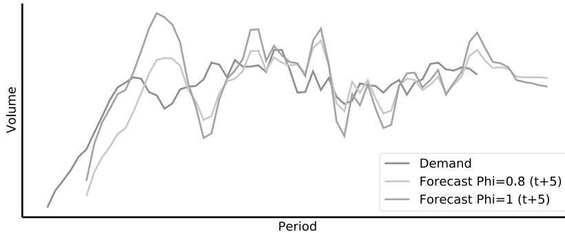
Figure 7.1: Forecast with damped trend.
