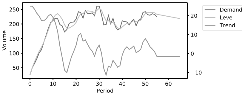
Figure 5.4: Level and trend components.
