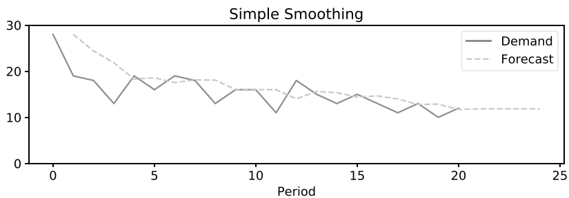
Figure 3.8: Example of simple smoothing forecast.
