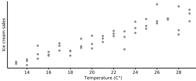
Figure 20.2: “My sales are linearly correlated to temperature!”
