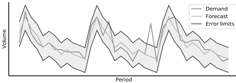
Figure 10.8: Outlier detection via forecast error.
