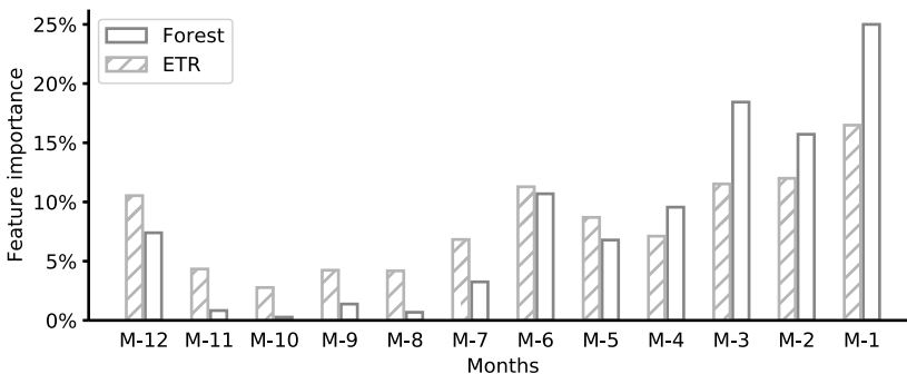
Figure 18.1: Feature importance.
