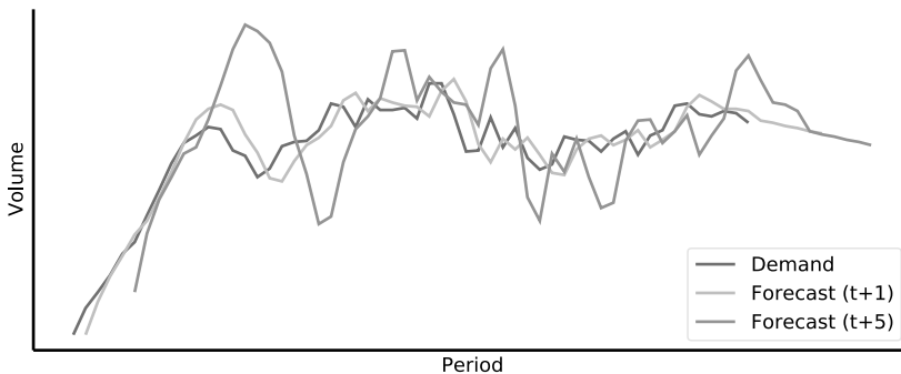
Figure 5.1: Forecast with \alpha = 0.2 and \beta = 0.4 .
