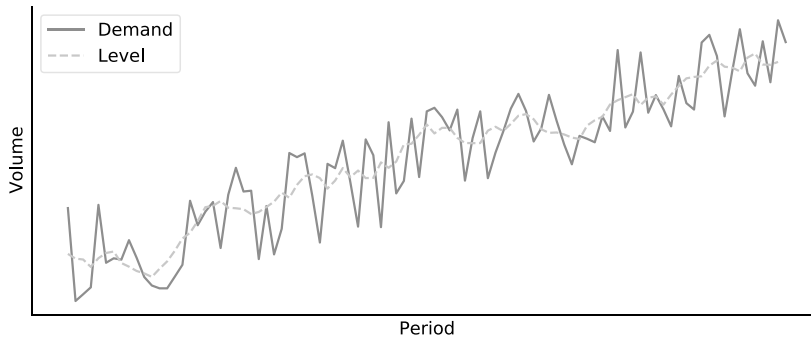
Figure 3.1: Demand level estimation.
