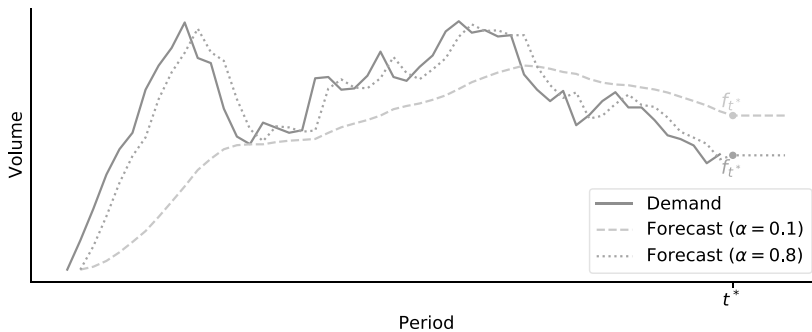
Figure 3.4: Simple exponential smoothing model.
