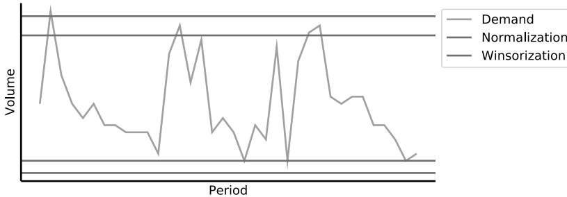
Figure 10.6: Winsorization and normalization on seasonal dataset.
