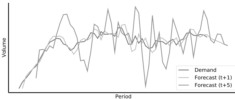
Figure 5.3: Forecast with \alpha = 0.8 and \beta = 0.8 .
