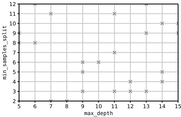
Figure 14.3: Random search.
