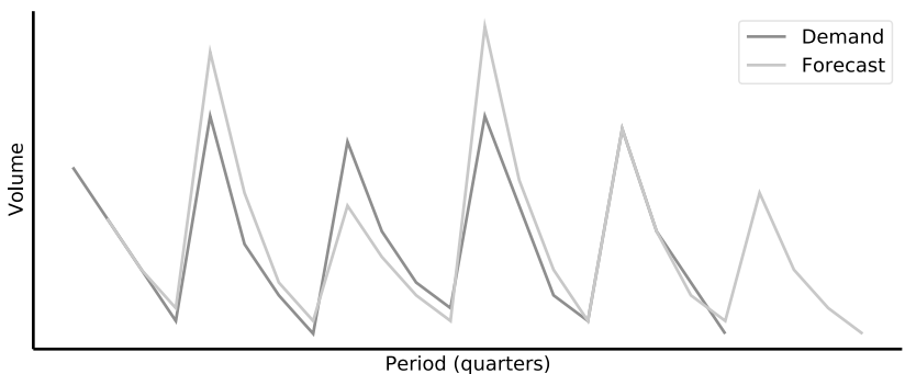
Figure 9.4: Quarterly forecast.
