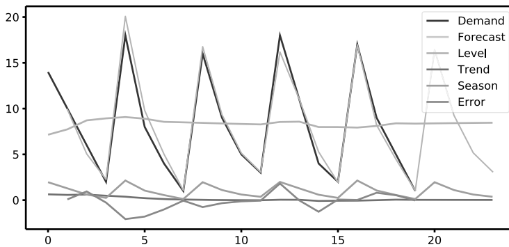
Figure 9.8: Messy graph of our time series.
