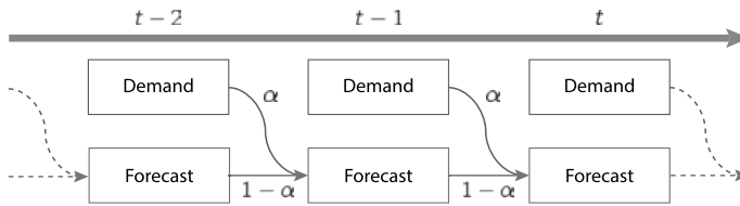
Figure 3.2: Simple exponential smoothing algorithm.
