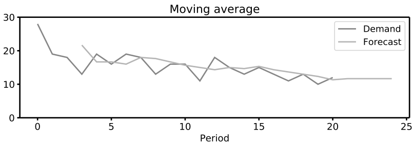
Figure 1.3: .plot() output.
