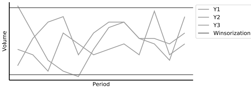
Figure 10.1: Winsorization on simple dataset.
