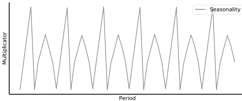
Figure 9.2: Seasonal factors.
