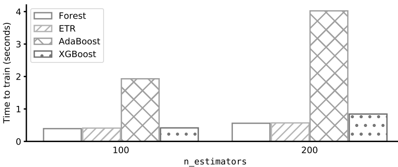
Figure 21.3: Impact of n_estimators on running time (using optimal parameters).
