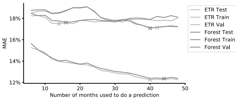
Figure 18.3: Feature optimization: Validation set.
