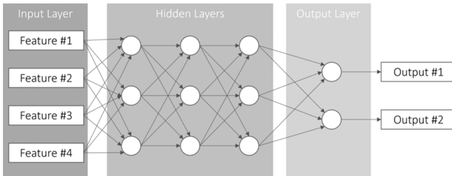
Figure 25.4: Example of neural network with four features, two outputs, and three hidden layers of 3 neurons (biases are not shown for the sake of simplicity).
