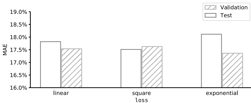
Figure 19.5: Loss function (with max_depth=8 , learning_rate=0.25 , n_estimators=100 ).
