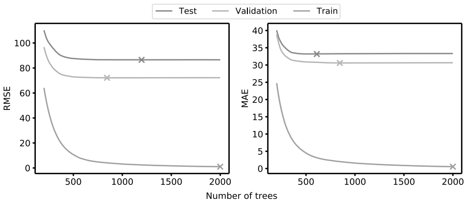
Figure 21.2: Early stopping using a validation set as an evaluation set.
