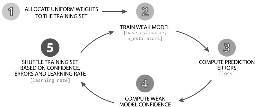
Figure 19.1: AdaBoost algorithm (with scikit-learn parameters).
