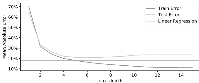
Figure 14.1: Experimentation for maximum depth optimization.
