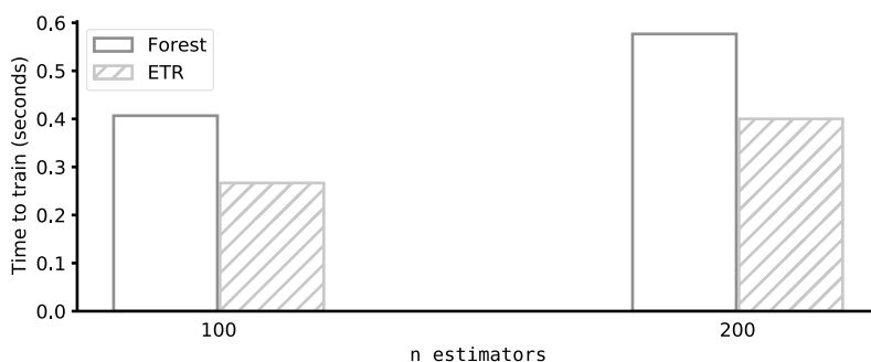
Figure 17.2: ETR vs. forest training time, both with the same parameters (optimal ones from Chapter 15).
