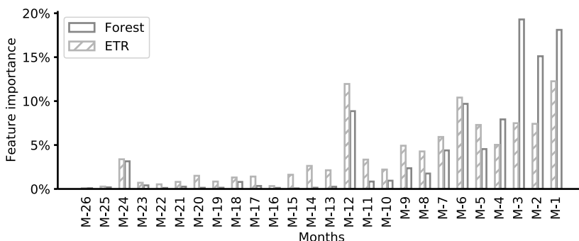
Figure 18.5: Feature importance for 26 months.
