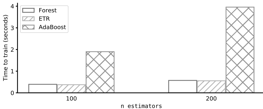
Figure 19.7: Impact of n_estimators on running time (using optimal parameters).
