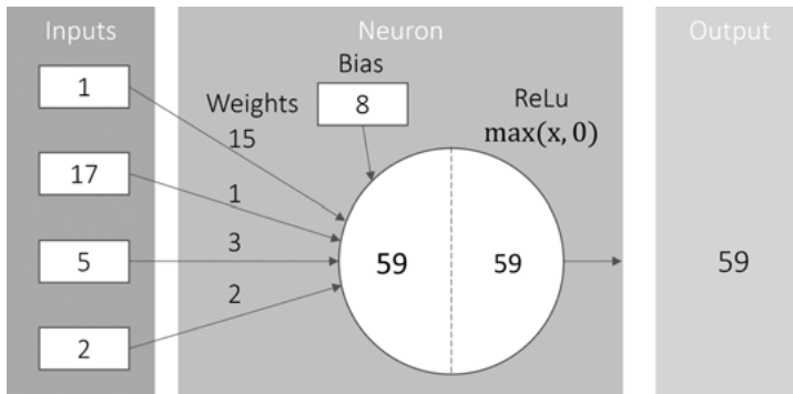
Figure 25.3: Example of a neuron using a ReLu activation function.
