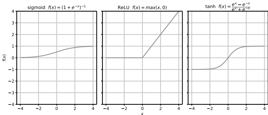
Figure 25.2: Most common activation functions.
