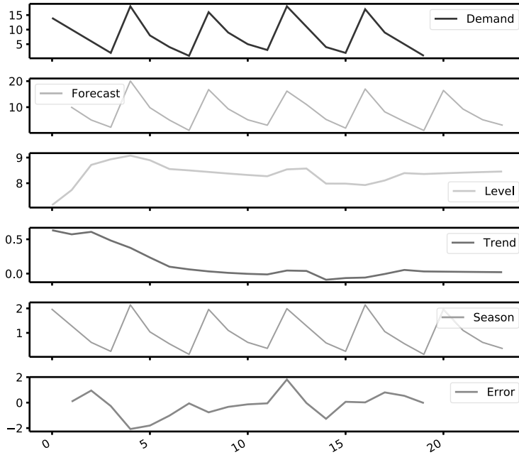
Figure 9.10: Subplots.
