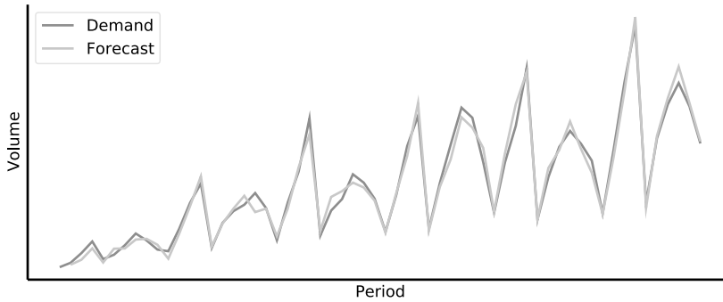
Figure 9.1: Example for seasonal forecast.
