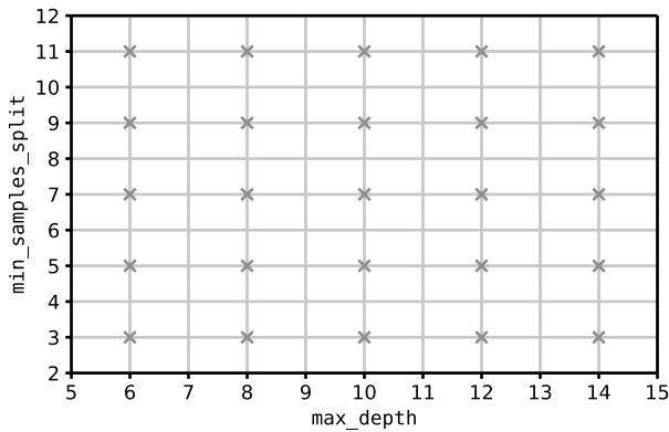
Figure 14.2: Grid search.
