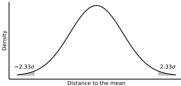
Figure 10.3: Normal curve excluding top and bottom 1% of values.
