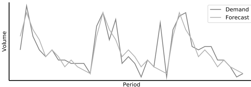
Figure 10.7: Seasonal demand.
