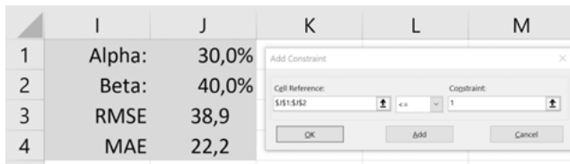
Figure 6.4: Add a constraint.
