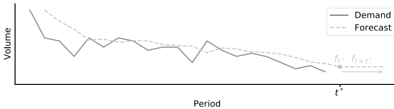
Figure 3.3: Future forecast with simple exponential smoothing.
