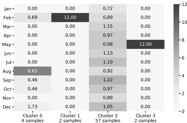
Figure 23.3: Cluster visualization.
