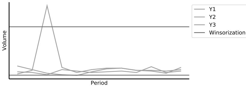
Figure 10.2: Winsorization on an extreme dataset.
