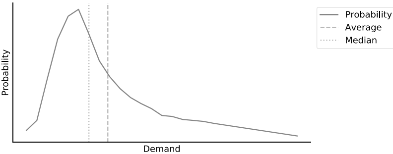
Figure 2.7: Median vs. Average.
