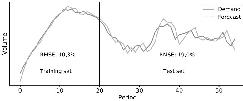
Figure 8.1: Overfitting.
