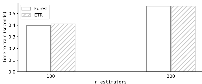
Figure 17.3: ETR vs. forest training time, both with their respective optimal parameters.
