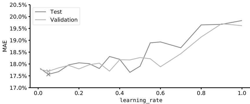
Figure 19.4: Learning rate impact (with n_estimators=100 , max_depth=8 , loss='linear' ).
