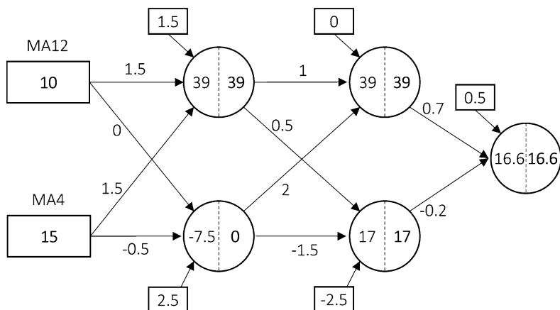
Figure 25.5: Example of forward propagation.
