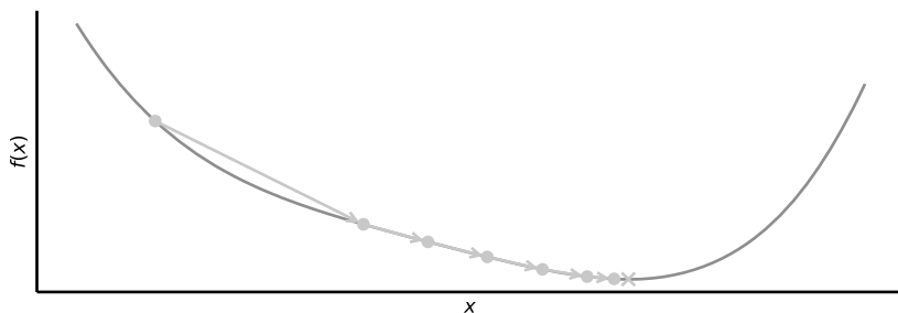
Figure 25.6: Example of gradient descent (first six steps).
