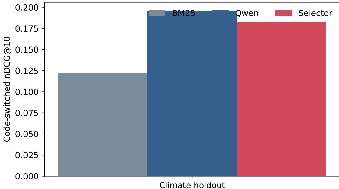
Frozen method performance (ArguAna not authorized by source gate)
