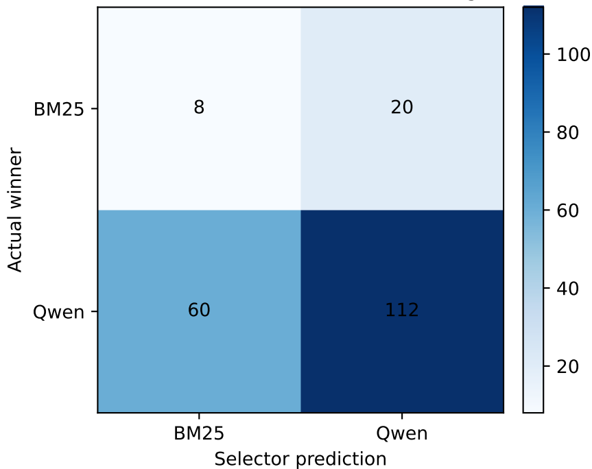
POST-HOC: Climate holdout routing
